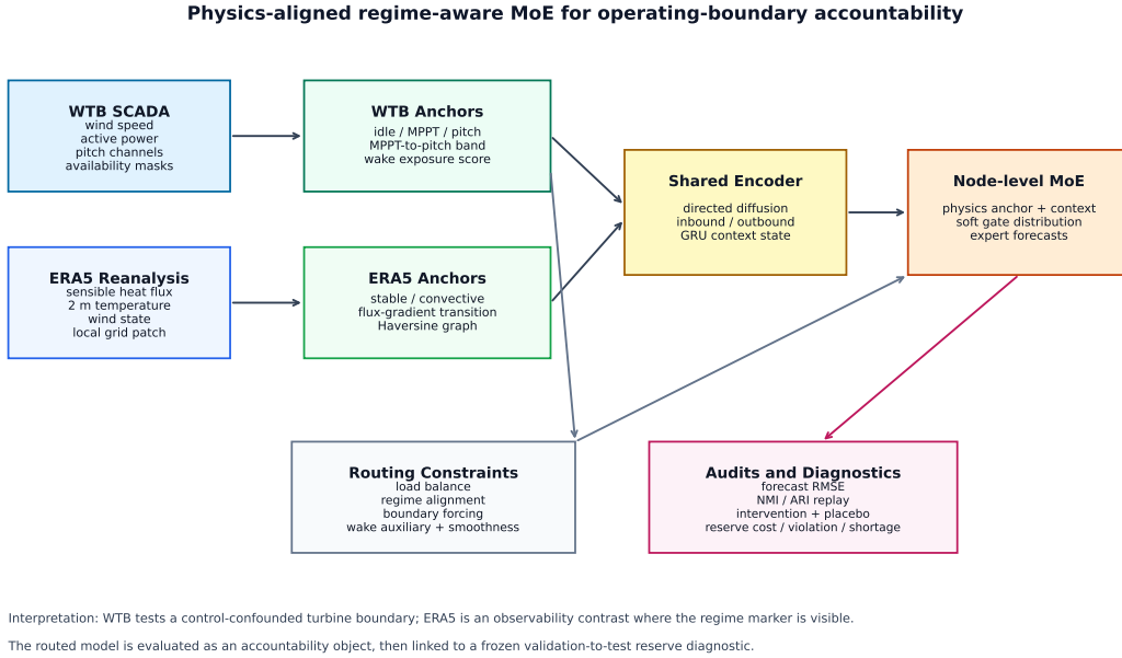
Figure 1: Physics-aligned regime-aware MoE. The two datasets share the same directed-diffusion GRU encoder and node-level MoE routing mechanism. WTB uses a dynamic wake graph and a boundary-focused forcing term, whereas ERA5 uses a Haversine-Gaussian graph and a thermodynamic regime anchor.
