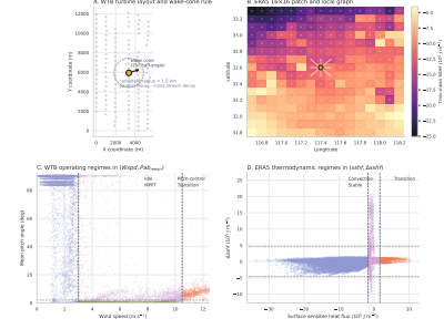
Fig. 1. Operating-decision context and physical regime anchors: (A) WTB layout with wake cone geometry; (B) ERA5 patch with sensible heat flux; (C) WTB operating regimes in ( Wspd , Pab_{mean} ) plane with MPPT-to-pitch boundary; (D) ERA5 thermodynamic regimes in ( sshf , \Delta sshf ) plane.
