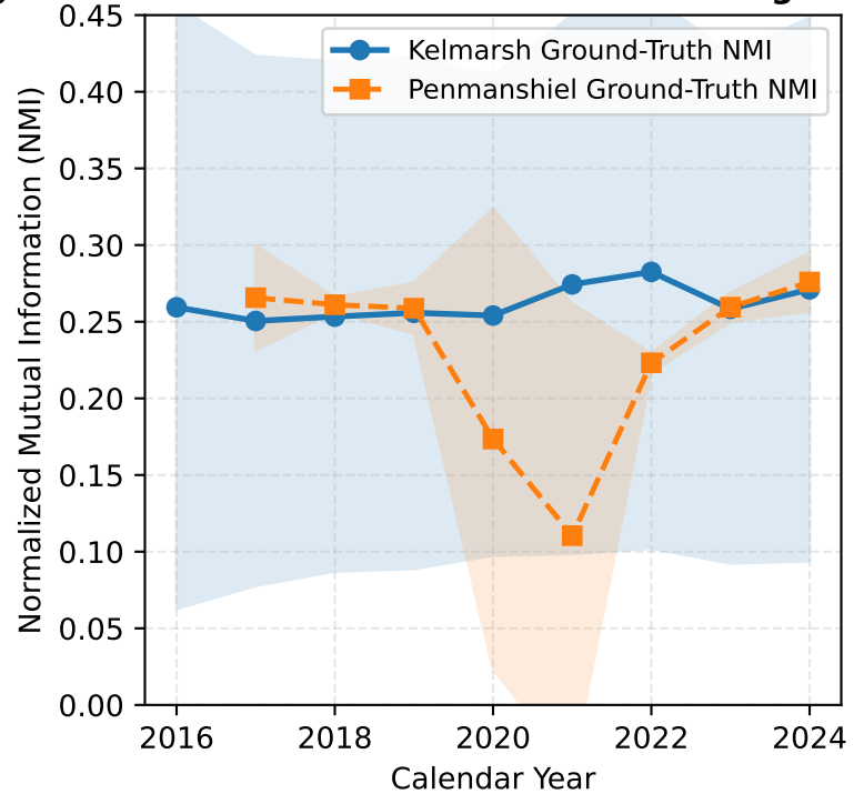
(c) Physical Boundary Alignment (NMI) Multi-Year Ground-Truth Tracking
