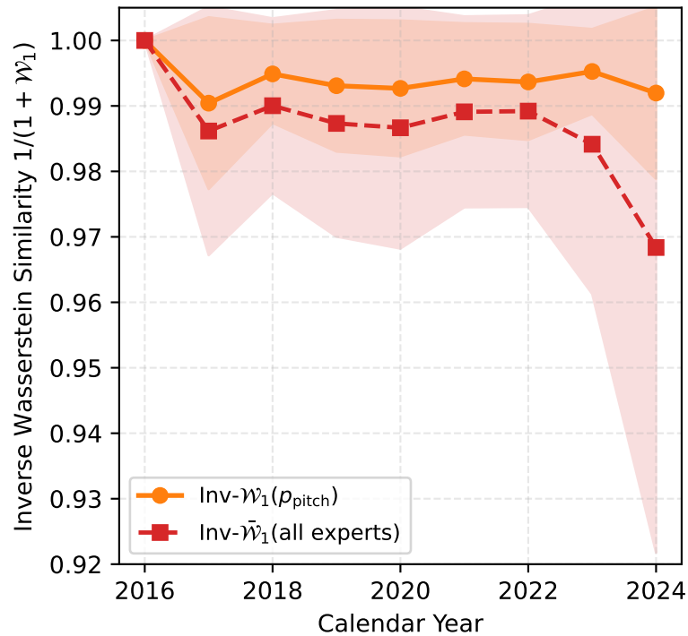
(b) Penmanshiel (8.6 Years, 15 Turbines) Representation Similarity vs Commissioning
