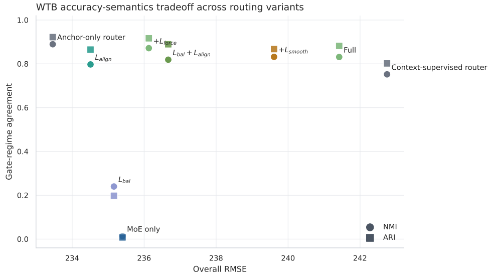
Figure 6: WTB accuracy-semantic tradeoff across routing variants. Circles show NMI and squares show ARI against overall RMSE. The frontier clarifies that stronger routing correction improves gate-regime agreement but can move the model away from the lowest forecast error.
