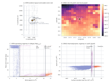
Fig. 1. Operating-decision context and physical regime anchors: (A) WTB layout with wake cone geometry ( 25^\circ half-angle); (B) ERA5 patch with sensible heat flux; (C) WTB operating regimes in (W_{\text{spd}}, P_{\text{ab\_mean}}) plane with MPPT-to-pitch boundary; (D) ERA5 thermodynamic regimes in (sshf, \Delta sshf) plane.
