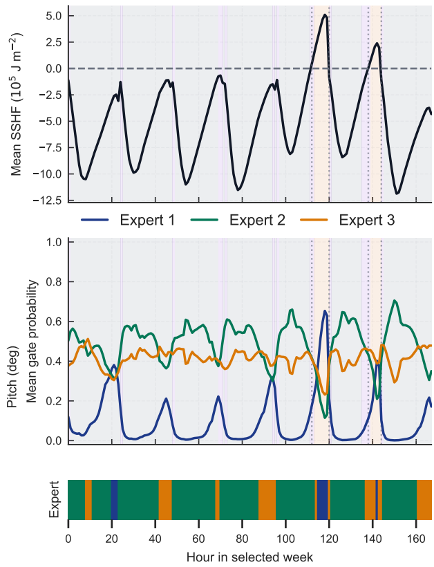
B. ERA5 weekly SSHF and expert weights
