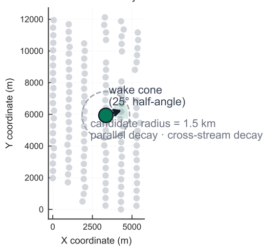
A. WTB turbine layout and wake-cone rule
