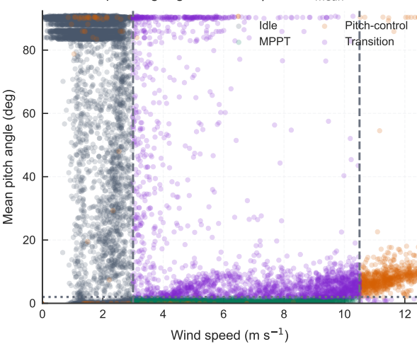
C. WTB operating regimes in ( Wspd, Pab_{mean} )
