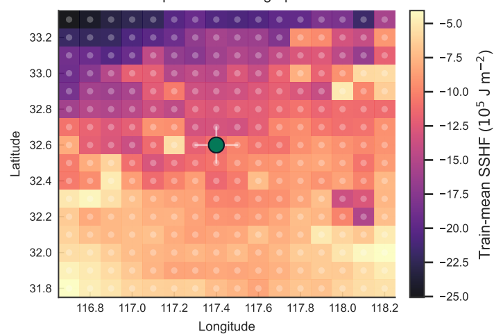
B. ERA5 16×16 patch and local graph
