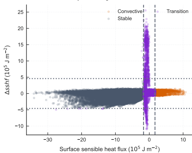
D. ERA5 thermodynamic regimes in ( sshf, \Delta sshf )
