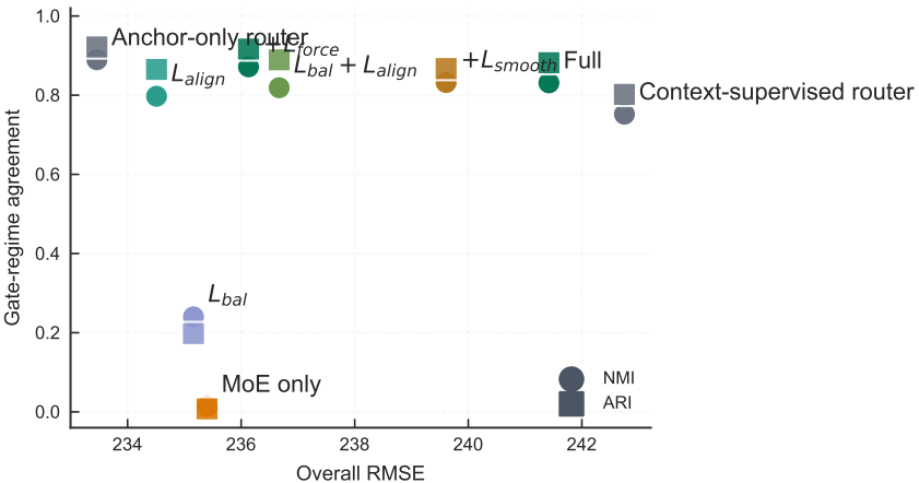
WTB accuracy-semantic tradeoff across routing variants
