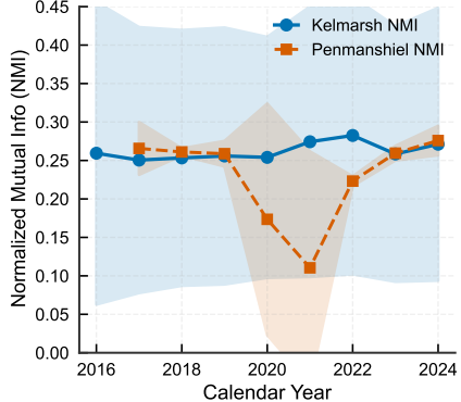
(c) Physical Boundary Alignment (NMI)
