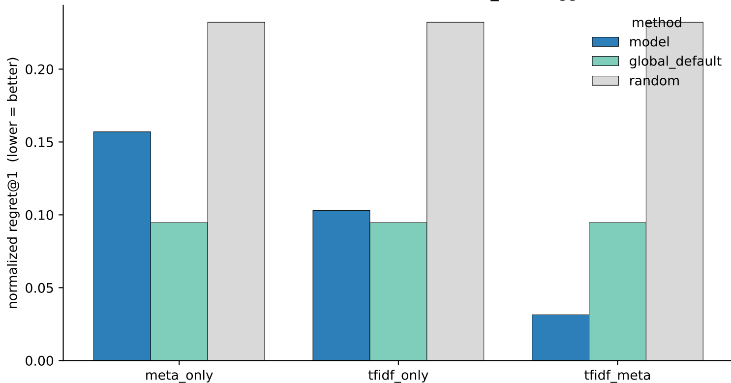
Zero-shot flow recommendation — extra_trees, agg=max
