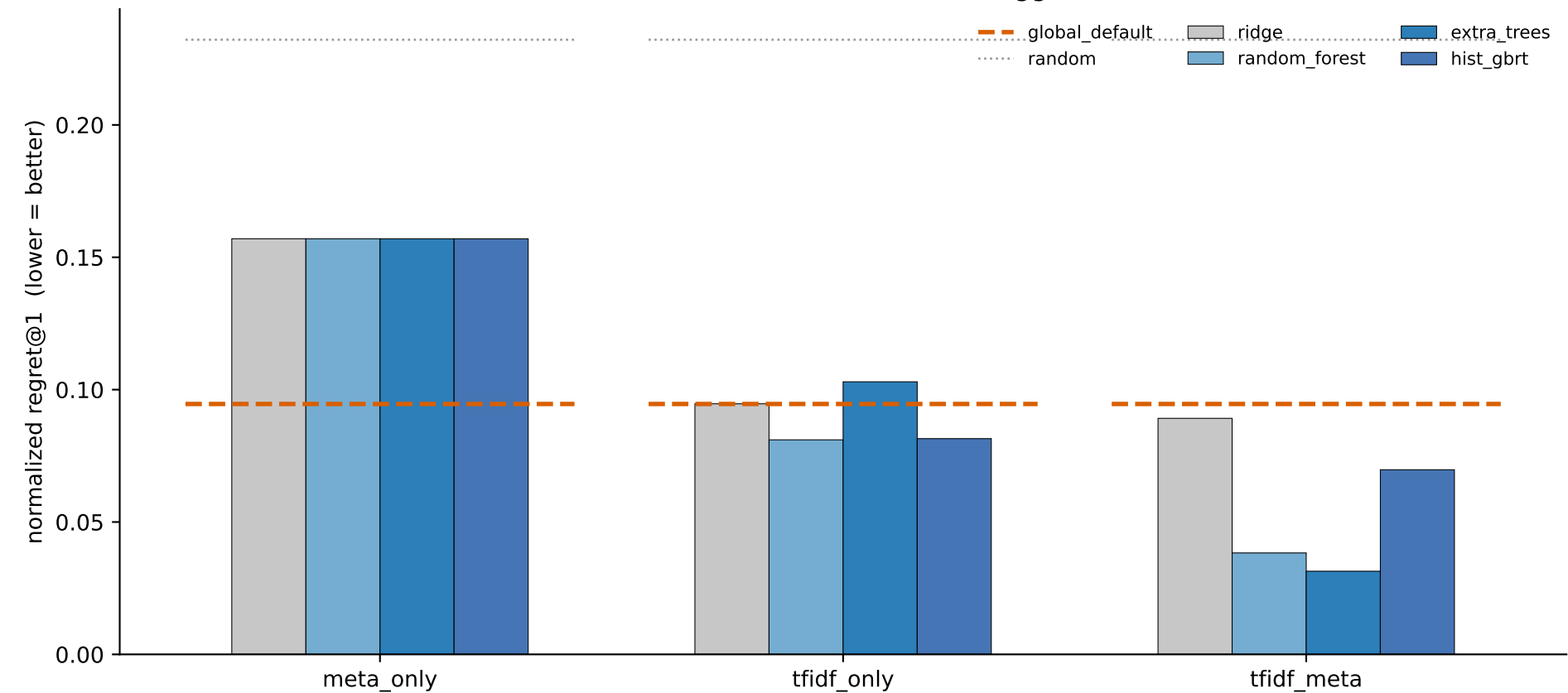
All models vs baselines — CC18, agg=max
