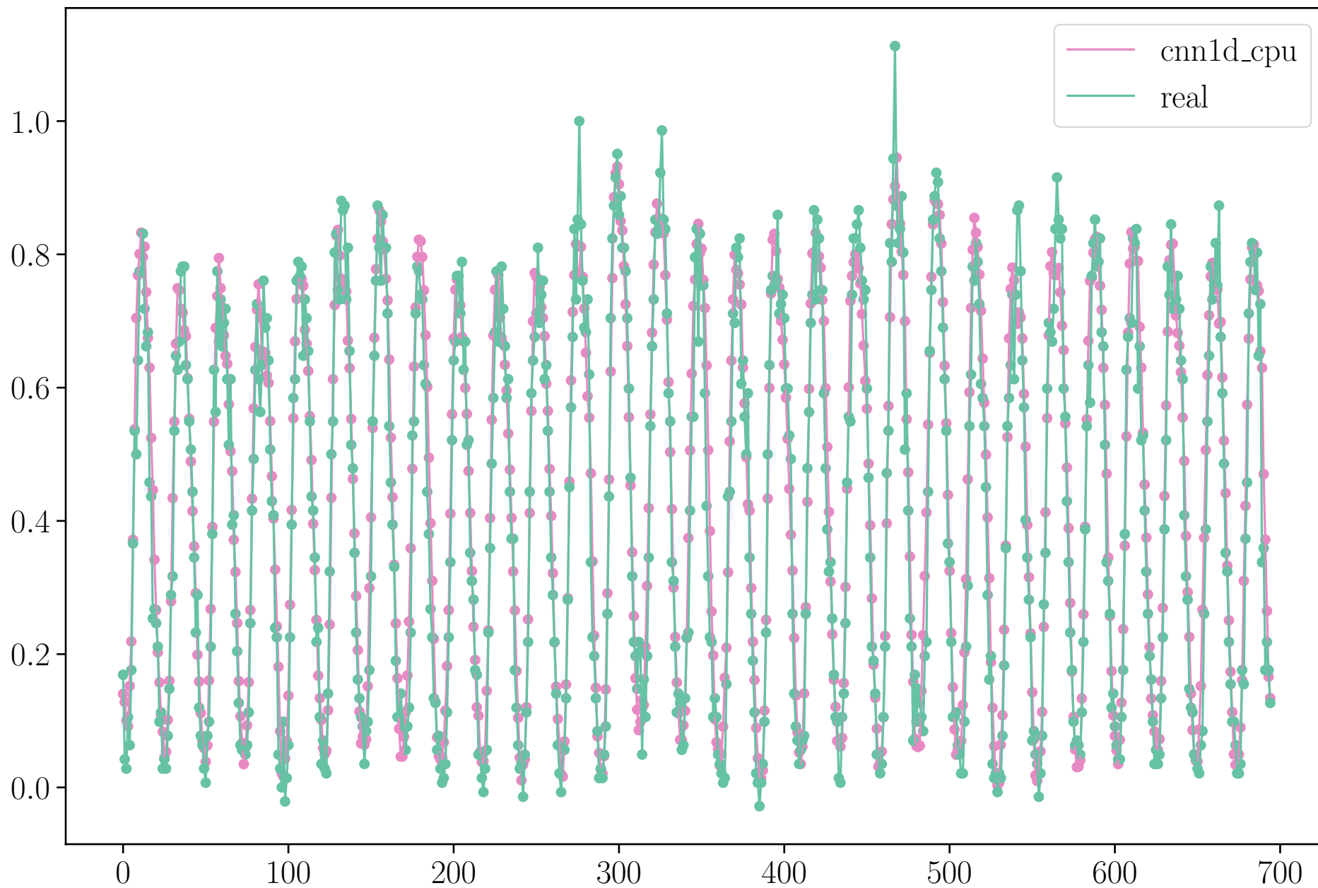
Predicted Values of CNN1D-CPU vs real values
