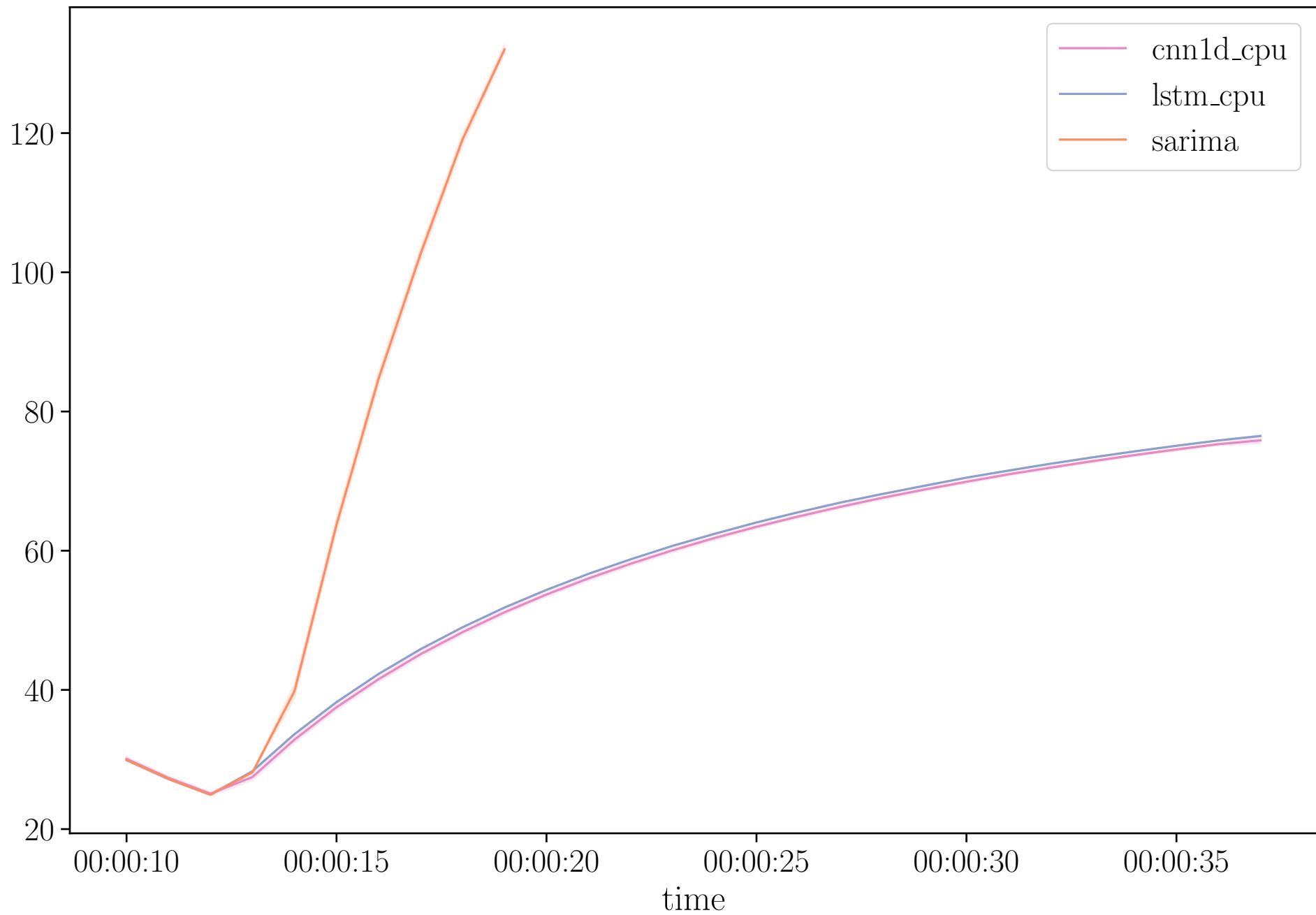
%CPU utilization
