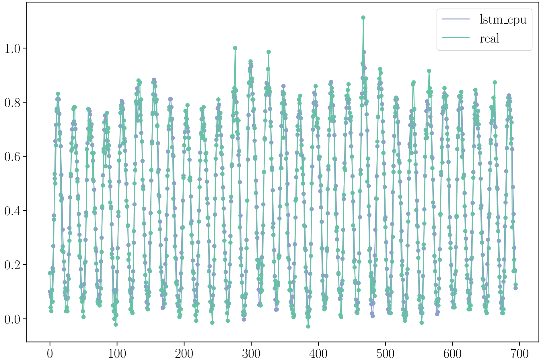
Predicted Values of LSTM-CPU vs real values
