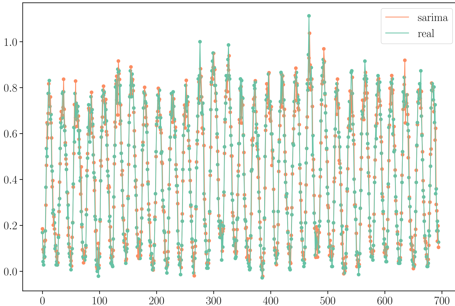
Predicted Values of SARIMA vs real values
