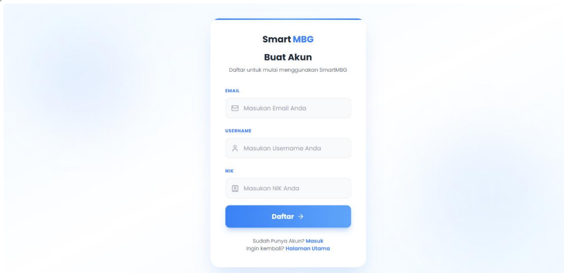
Gambar II. Halaman Sign-Up/Register.
