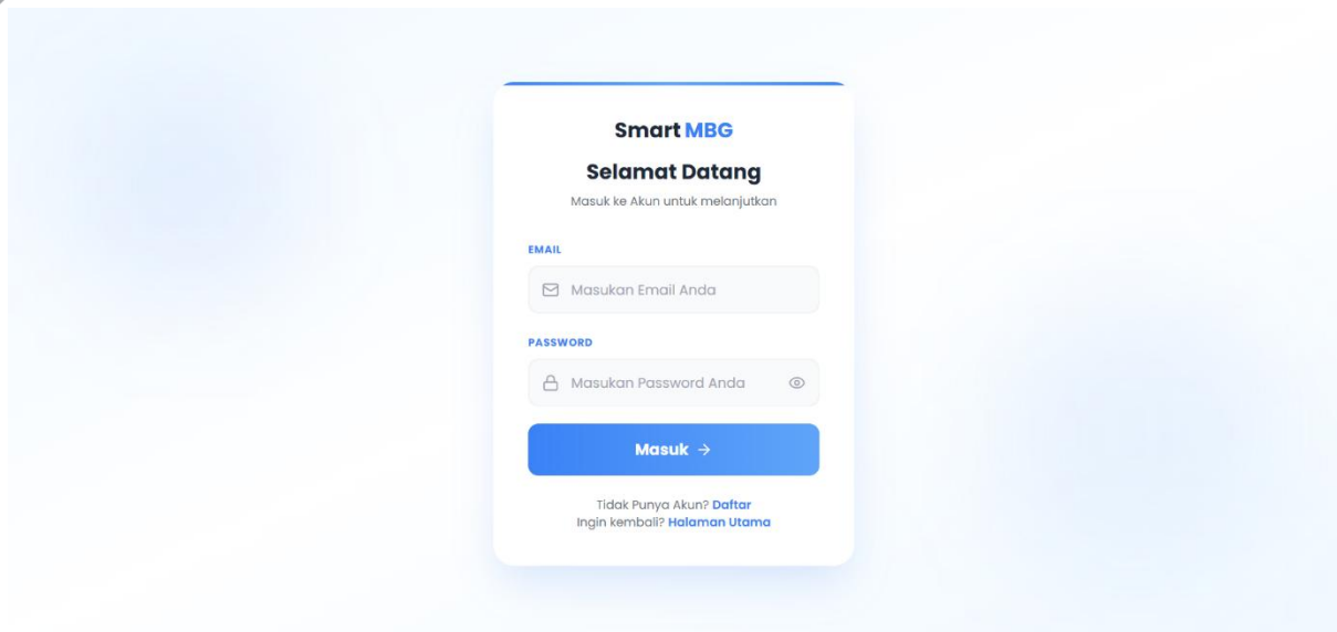
Gambar IV. Halaman Log-in.
