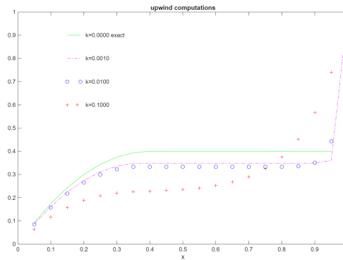
Figure 9: Upwind k = 0.1, 0.01, 0.001 .
