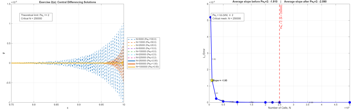
Figure 6: Influence of mesh resolution on central differencing using a Neumann outlet boundary condition. Left: numerical solution profiles near the outlet boundary. Right: convergence plot relative to the reference solution obtained with N = 10^6 .
