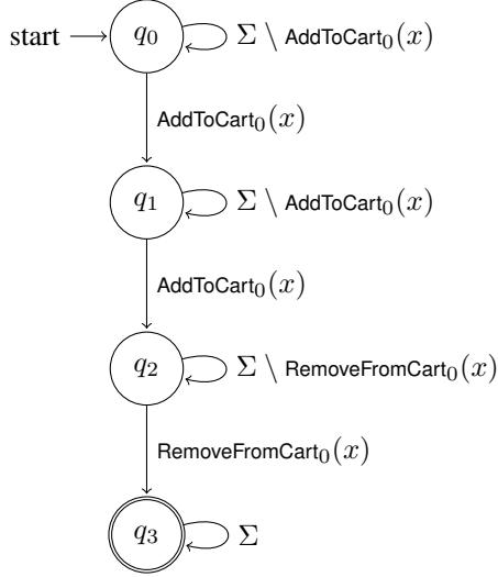
Fig. 2. An explanation DFA \mathcal{E} for the bug described in Example 1
