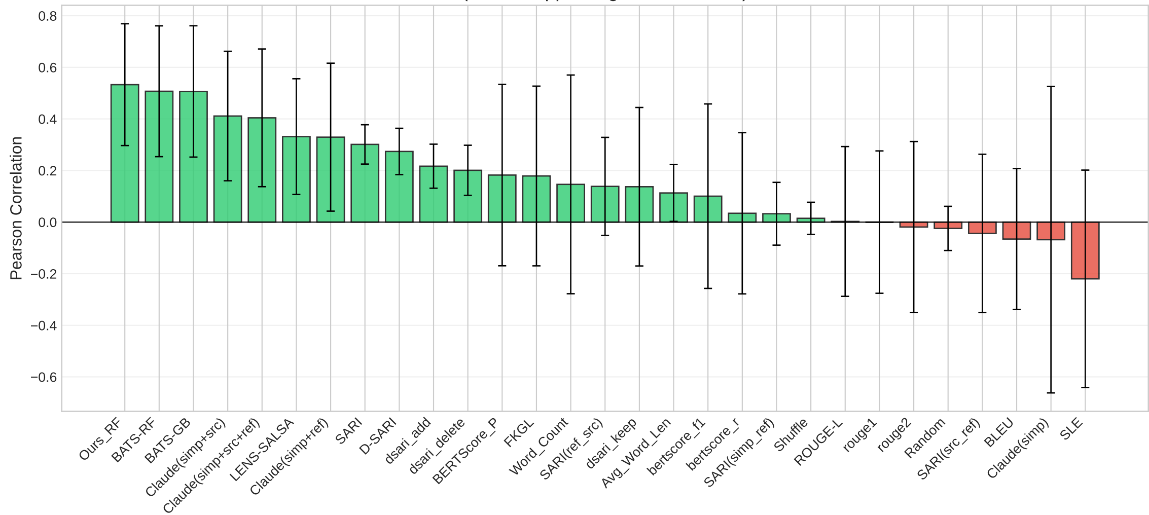
Metric Correlations: Mean \pm Std Across Datasets (Metrics appearing in 3+ datasets)
