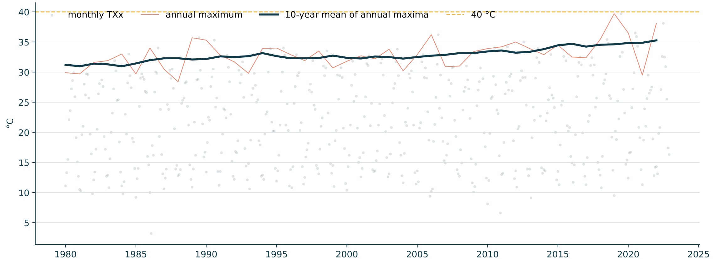
Evolution of monthly maximum daily temperature (TXx)
