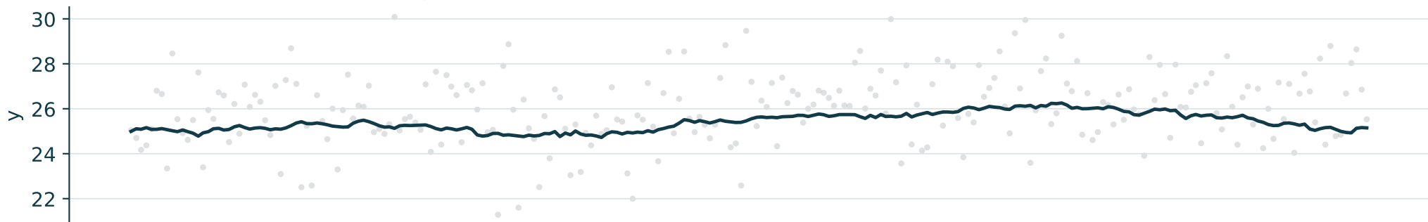
Stochastic local level — level=dynamic, slope=zero, seasonal=zero
