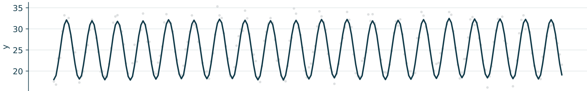
Local level + fixed season — level=dynamic, slope=zero, seasonal=fixed
