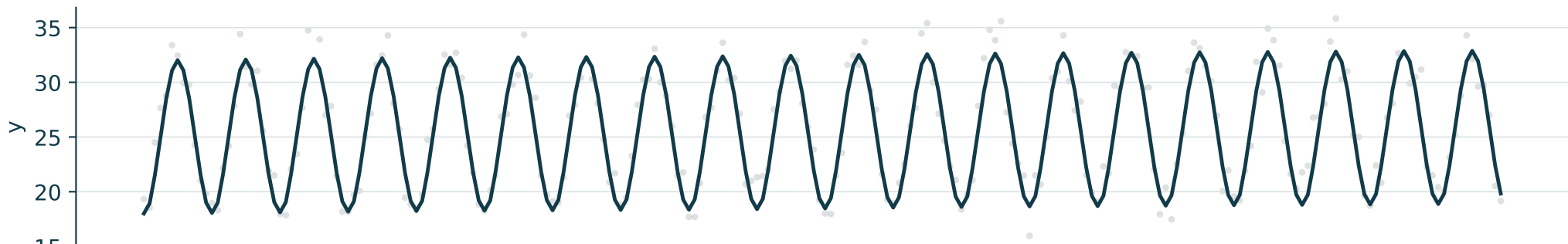
Stochastic trend + fixed season — level=fixed, slope=dynamic, seasonal=fixed
