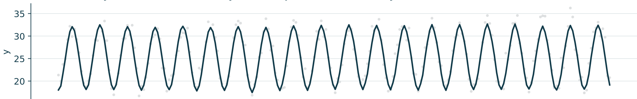
Local level + dynamic season — level=dynamic, slope=zero, seasonal=dynamic
