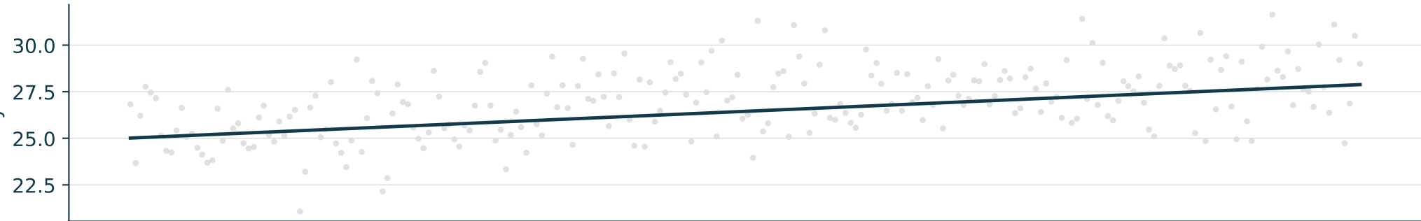
Fixed linear trend — level=fixed, slope=fixed, seasonal=zero
