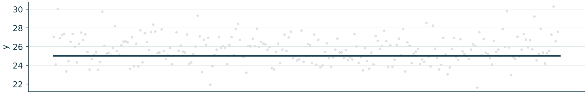
Stationary location — level=fixed, slope=zero, seasonal=zero
