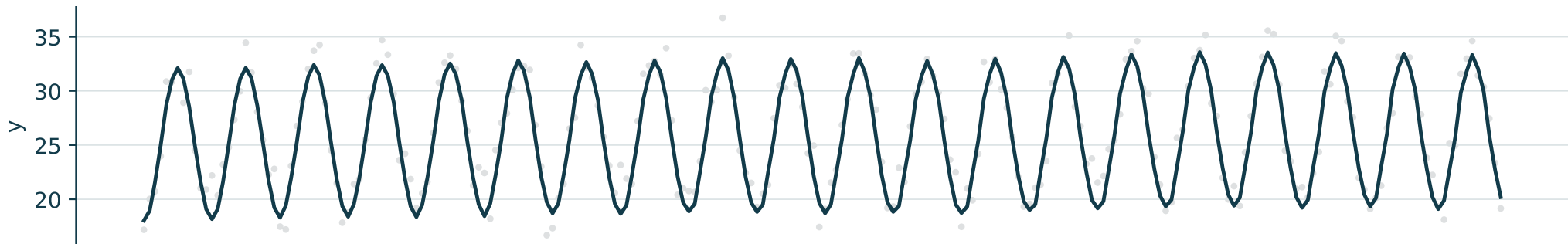
Level + trend + dynamic season — level=dynamic, slope=dynamic, seasonal=dynamic
