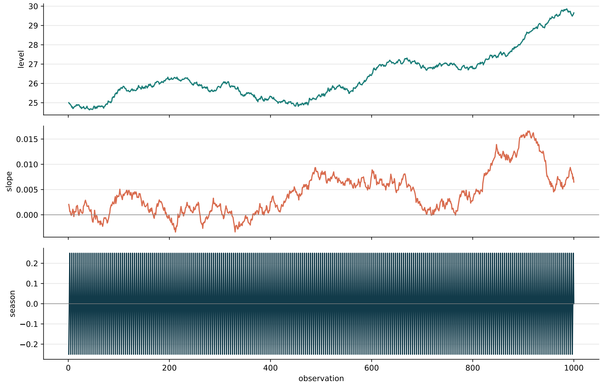
Local linear trend + fixed seasonality: structural decomposition
