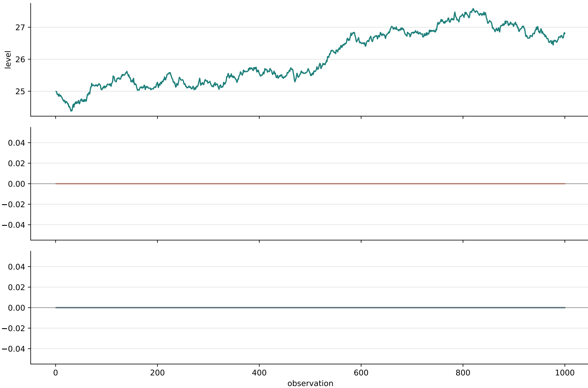
Random walk: structural decomposition
