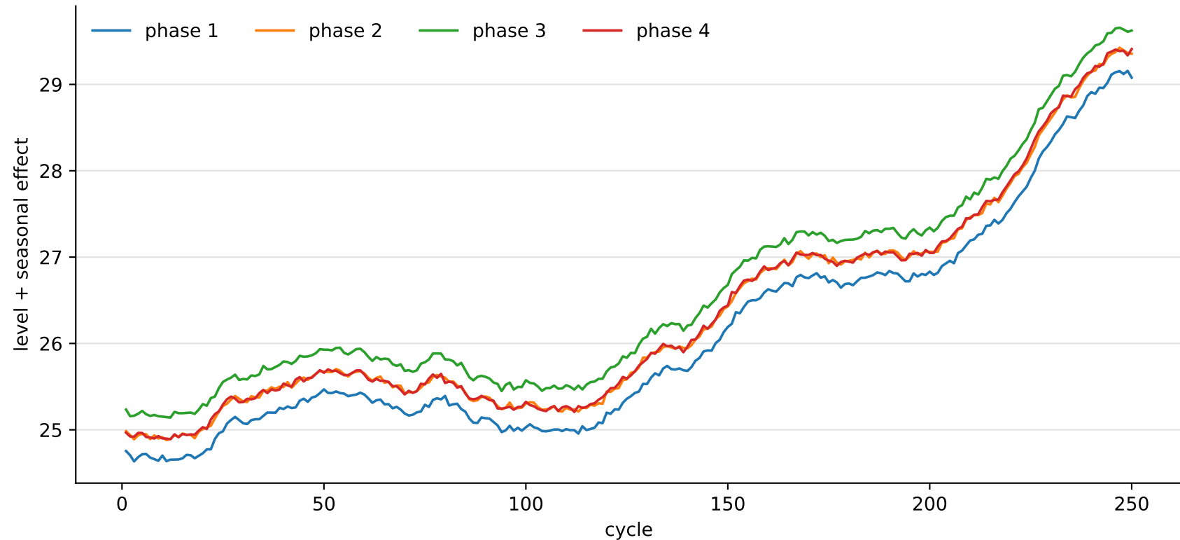
Local linear trend + fixed seasonality: phase-specific latent trajectories
