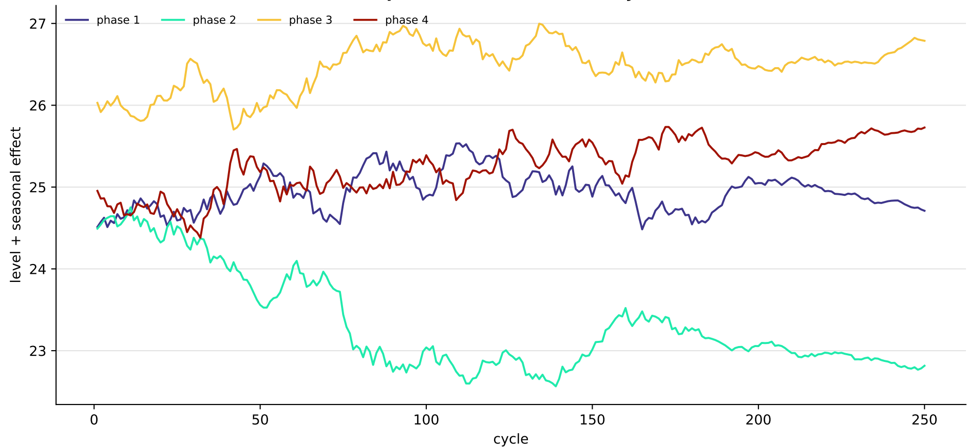
stationary_dynamic_season: phase-specific latent seasonal trajectories
