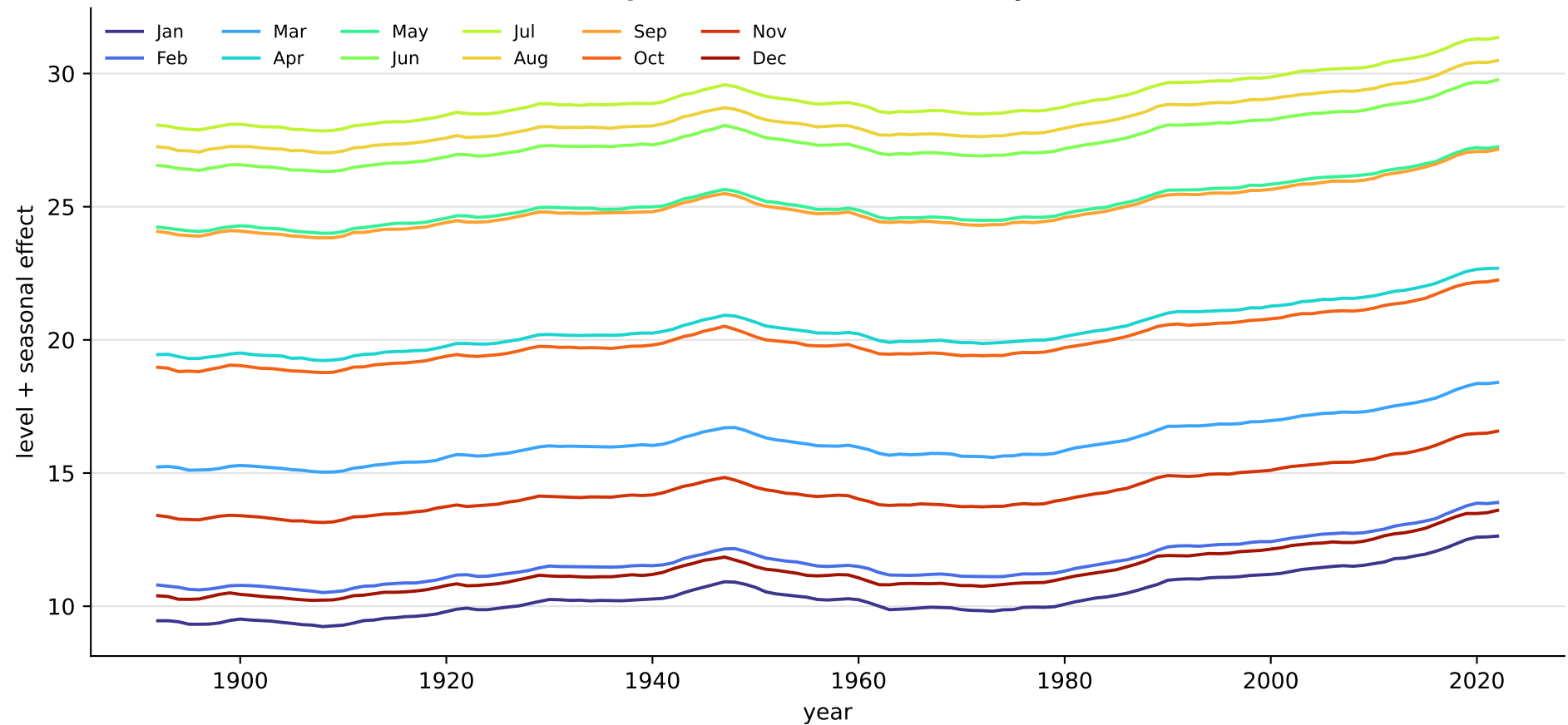
Phase-specific latent seasonal trajectories
