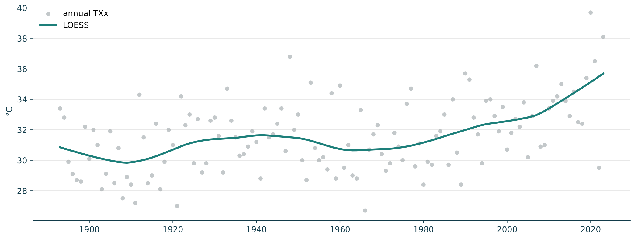
Evolution of annual maximum temperature (TXx)
