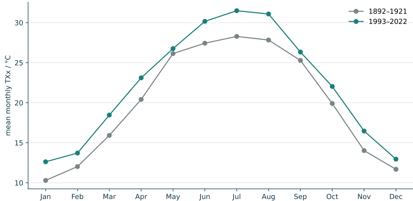
TXx seasonal cycle: early and recent climates
