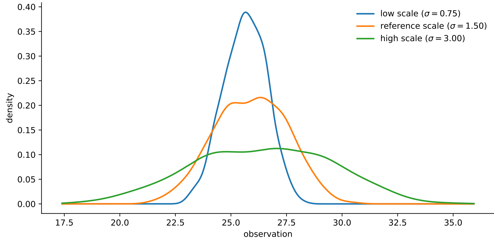
GEV scale comparison on a common latent path
