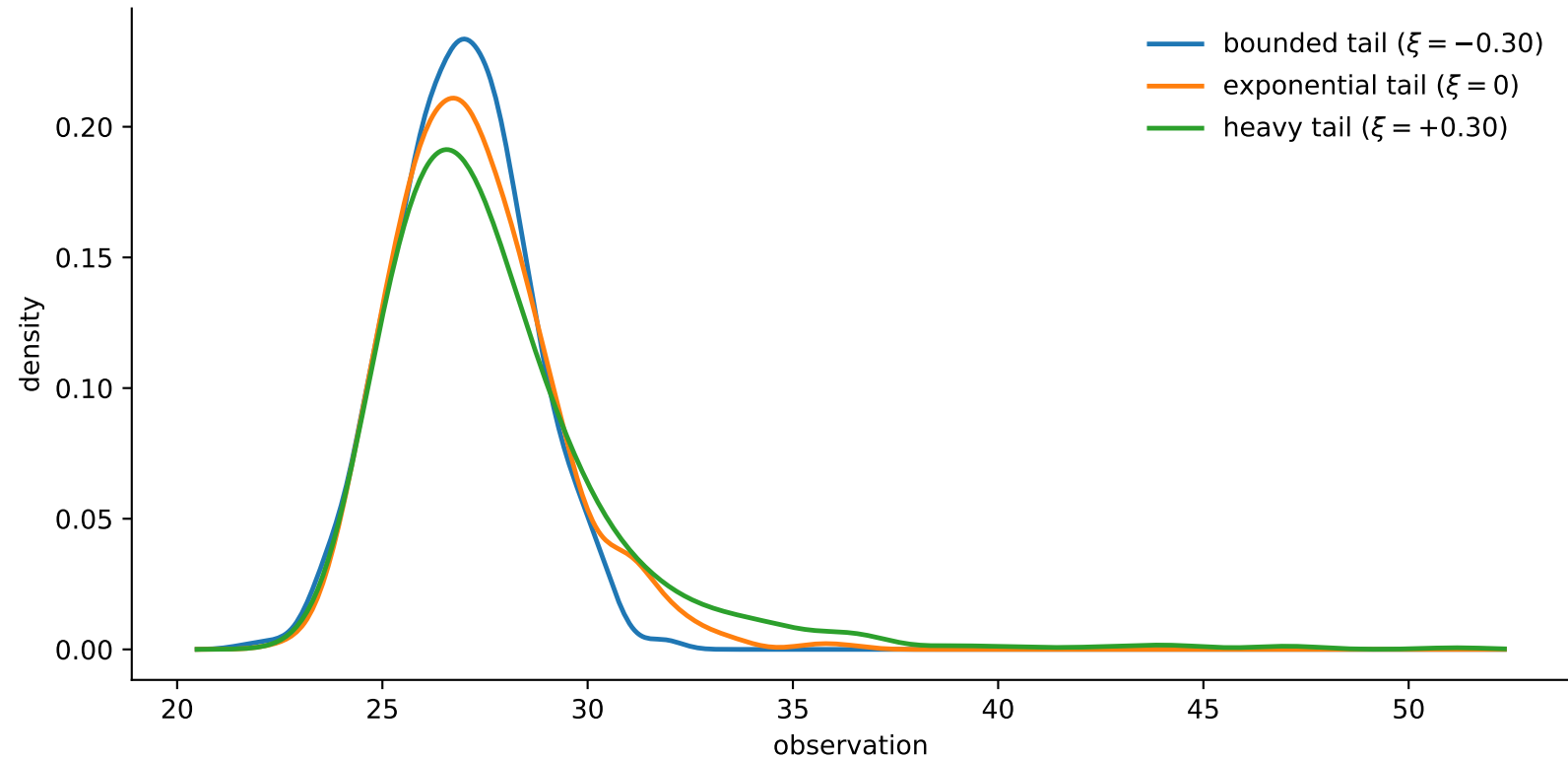
GEV shape comparison on a common latent path
