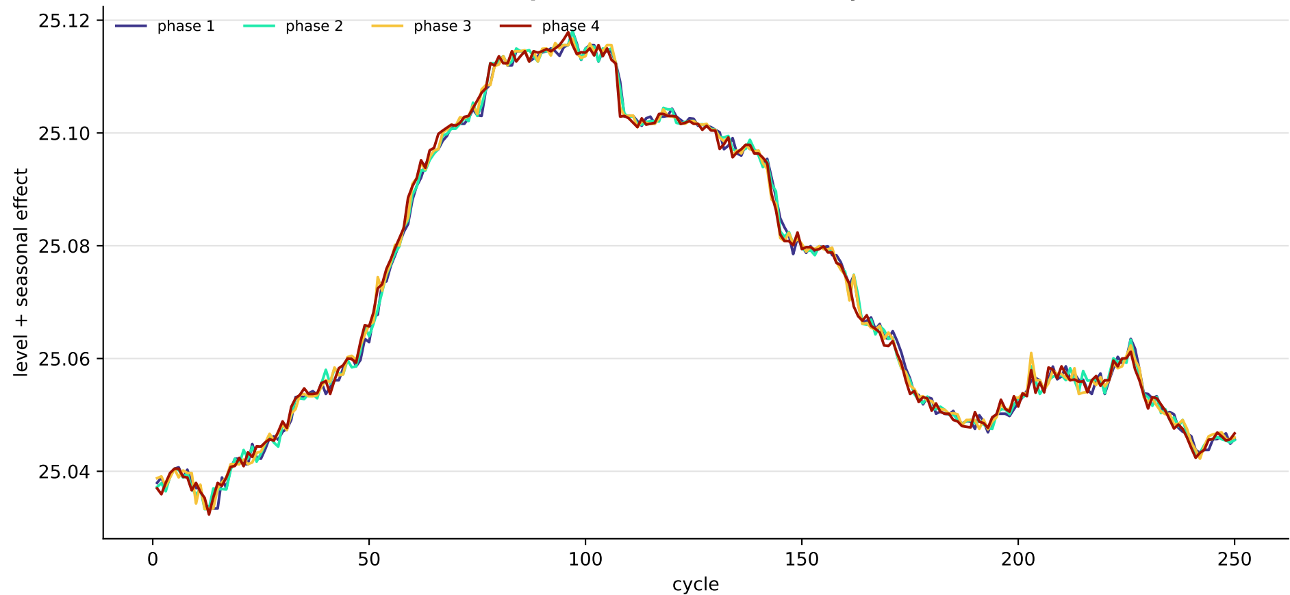
stationary: phase-specific posterior trajectories Phase-specific latent seasonal trajectories
