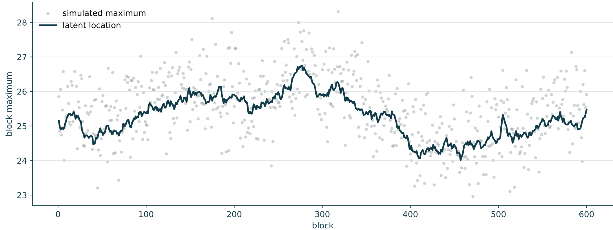
Low observation scale: \sigma=0.75 , \xi=-0.30
