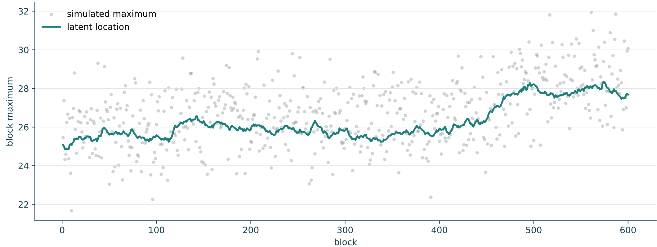
Local level, bounded tail: \xi=-0.30 , \sigma=1.50
