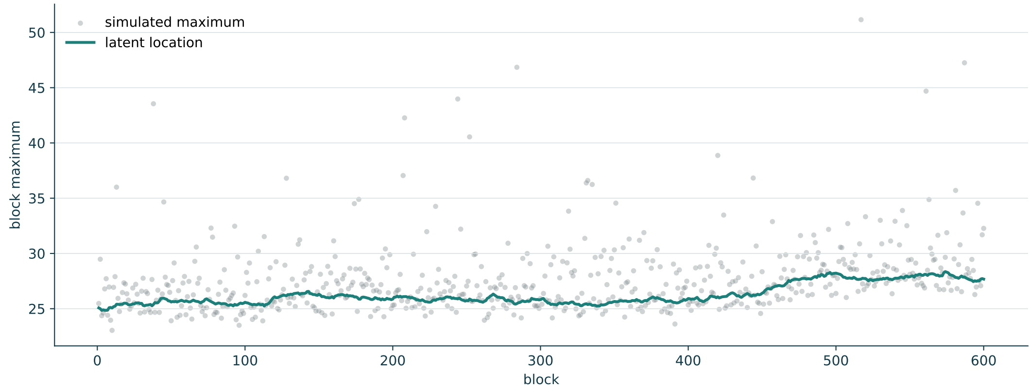
Local level, heavy tail: \xi=+0.30 , \sigma=1.50
