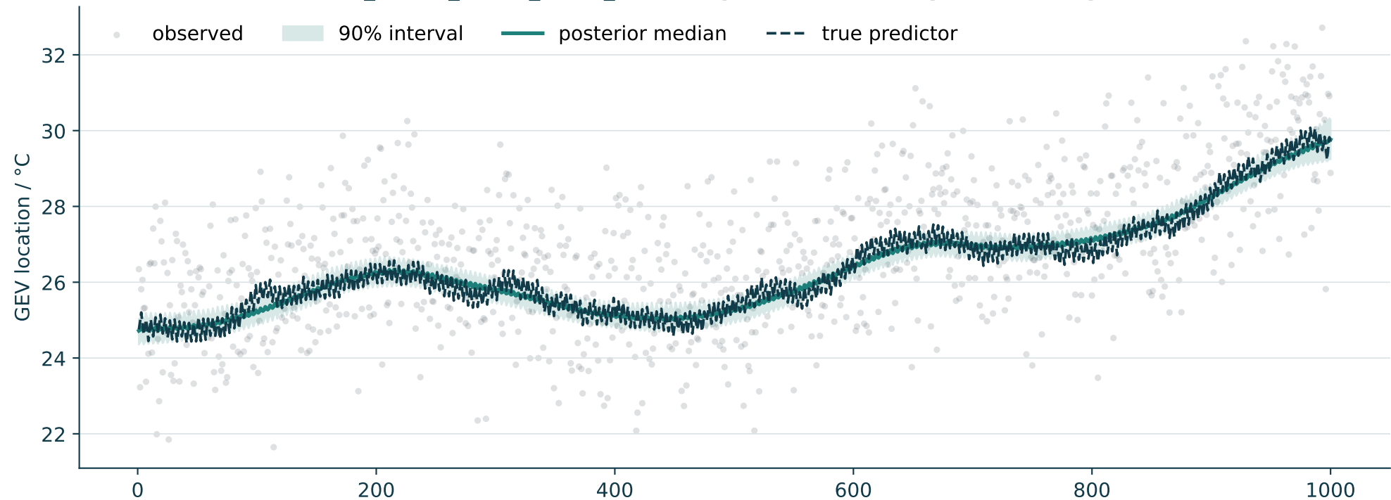
local_linear_trend_fixed_season: posterior latent predictor (laplace)
