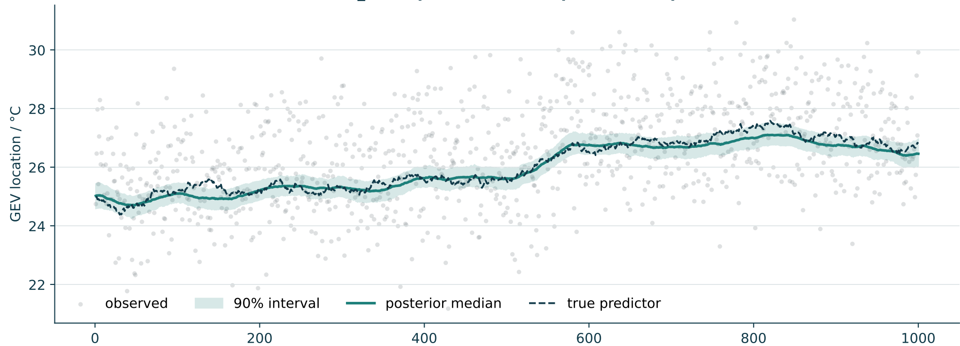
random_walk: posterior latent predictor (laplace)
