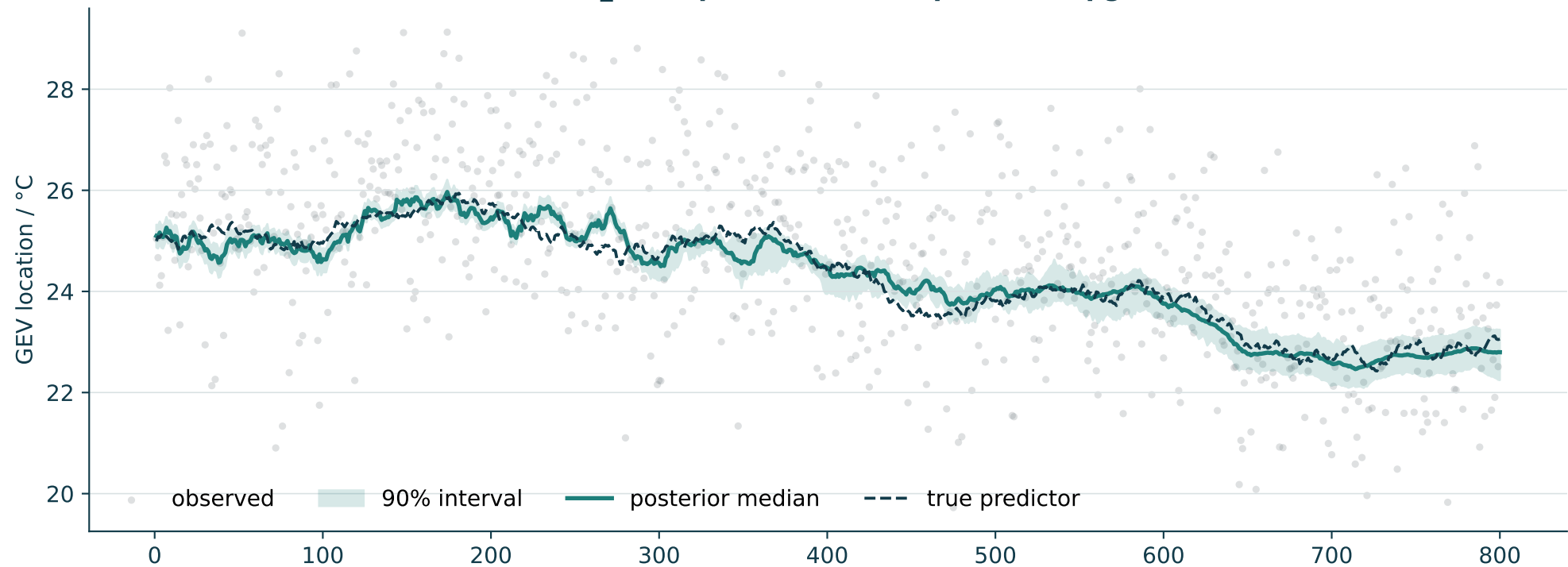
random_walk: posterior latent predictor (pgas)
