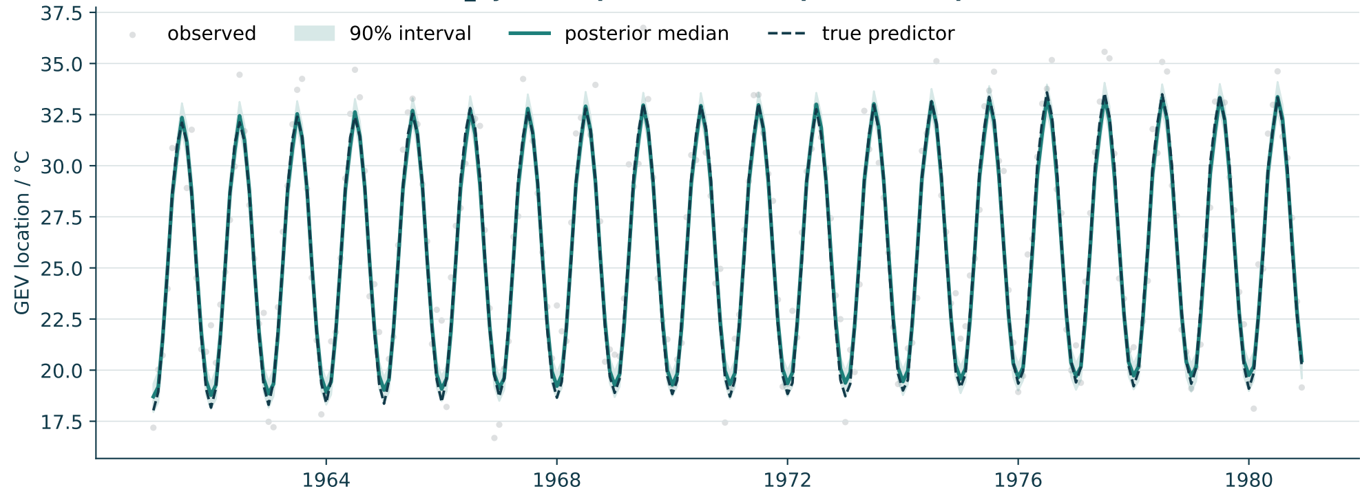
full_dynamic: posterior latent predictor (laplace)
