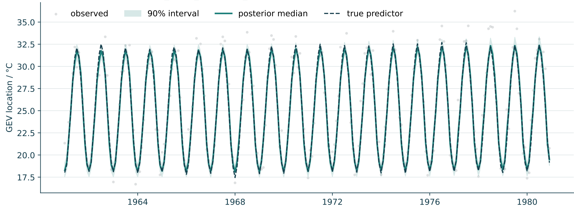
local_level_dynamic_season: posterior latent predictor (laplace)
