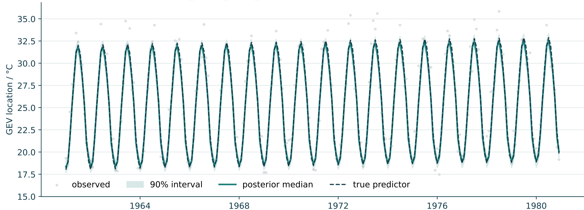
stochastic_trend_fixed_season: posterior latent predictor (laplace)
