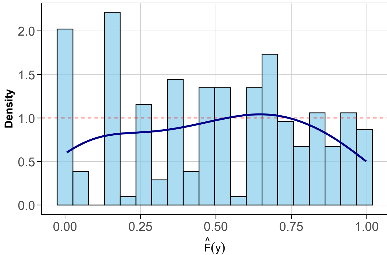
Uniformity Check of Transformed Exceedances
