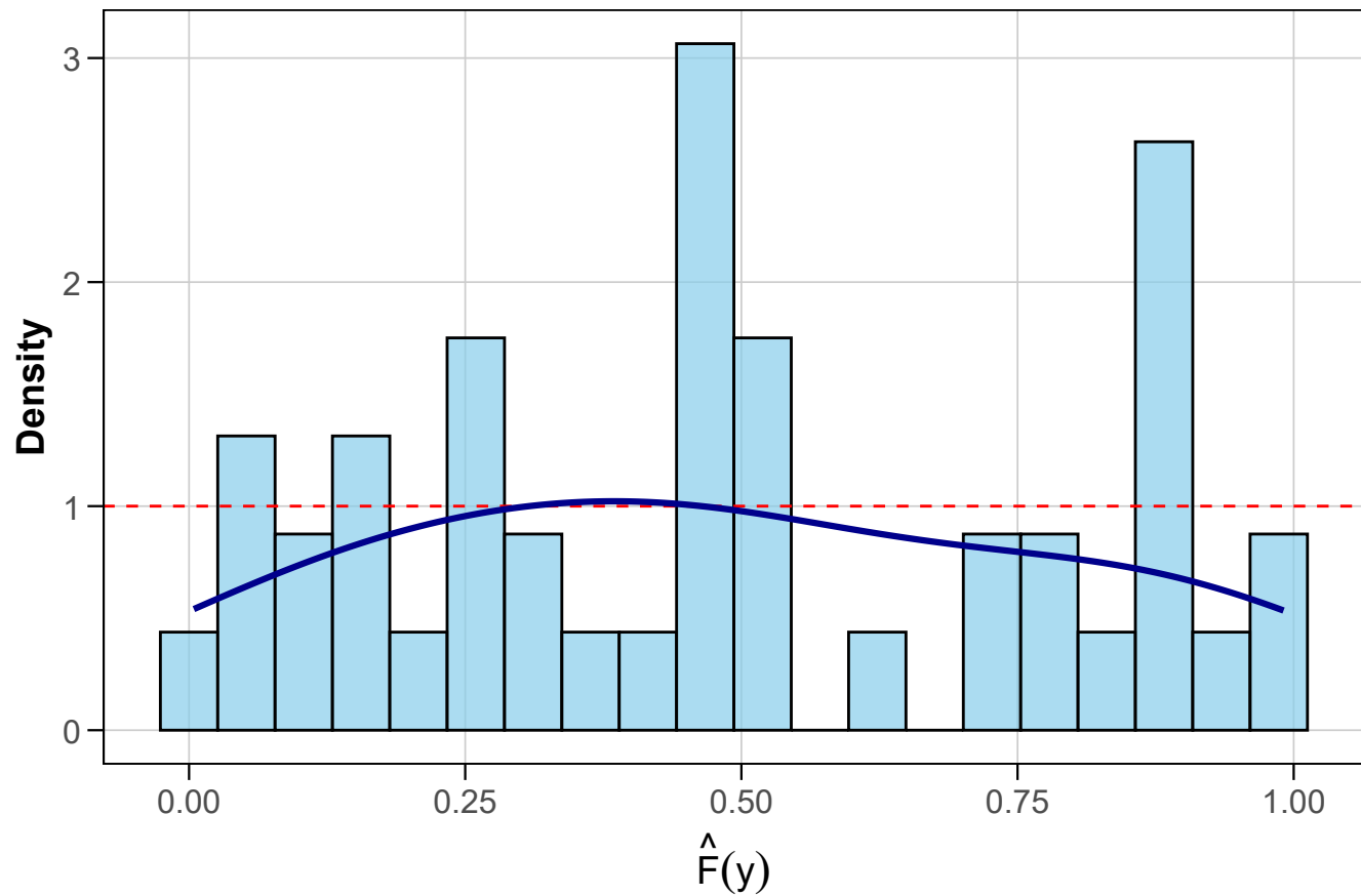
Uniformity: PIT (log CFH)
