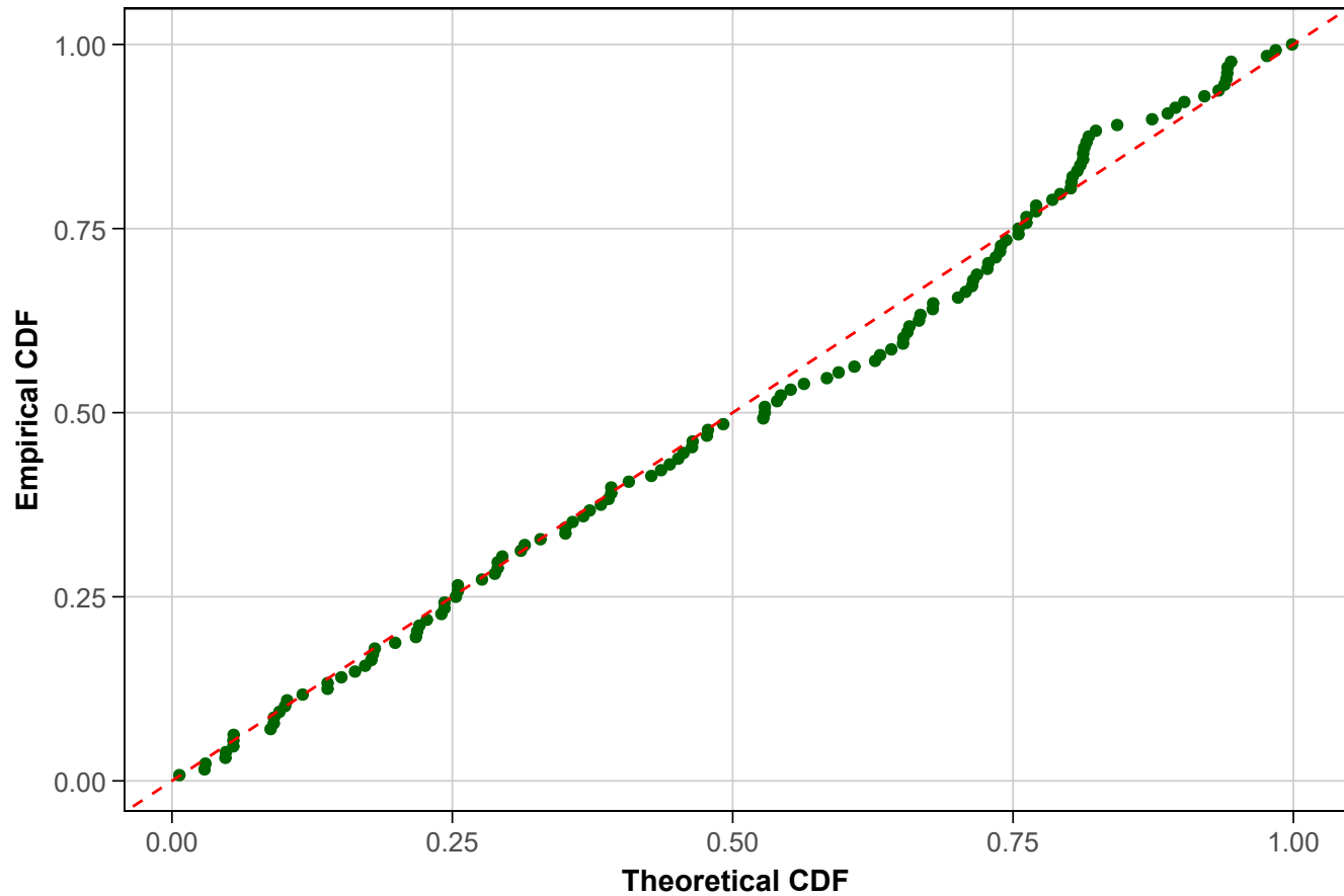
P-P Plot for GPD Fit
