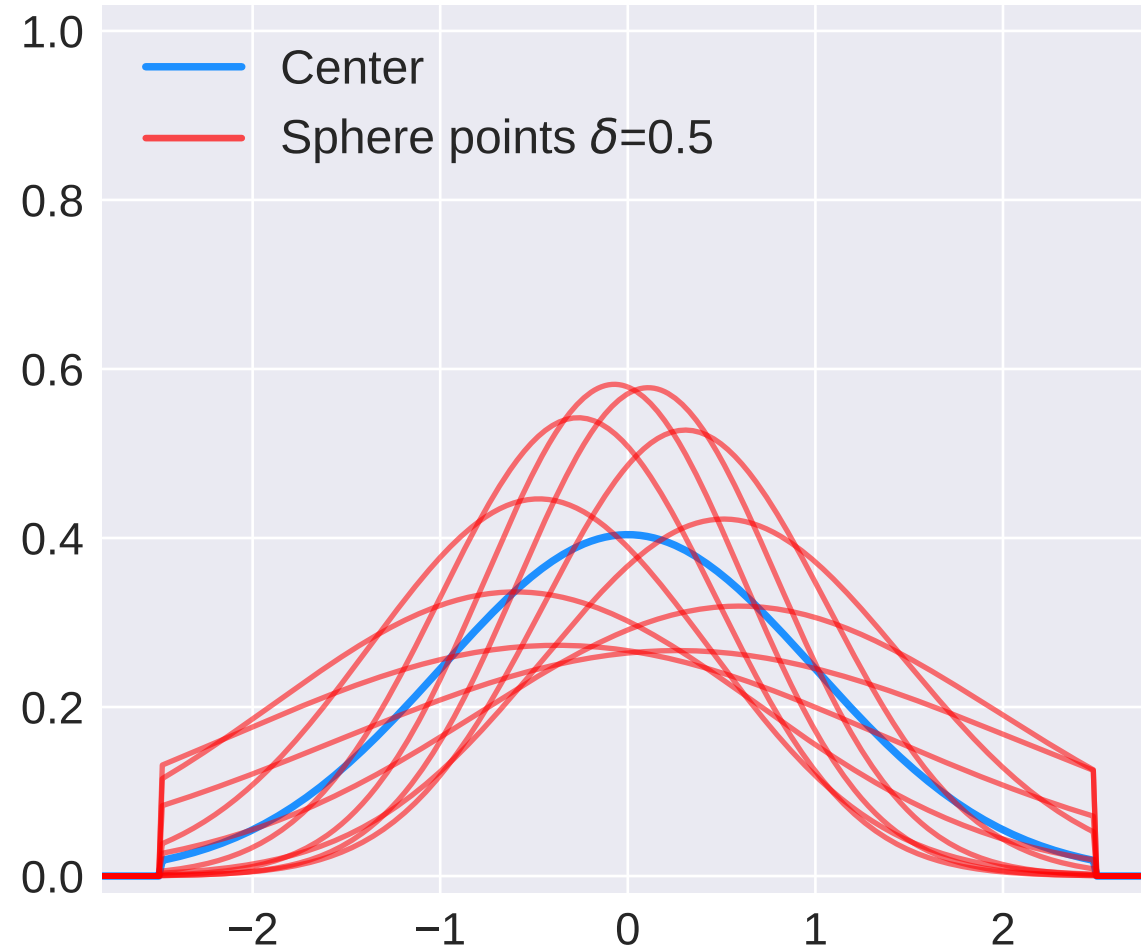
Normal distributions tr. on [-2.5, 2.5]
