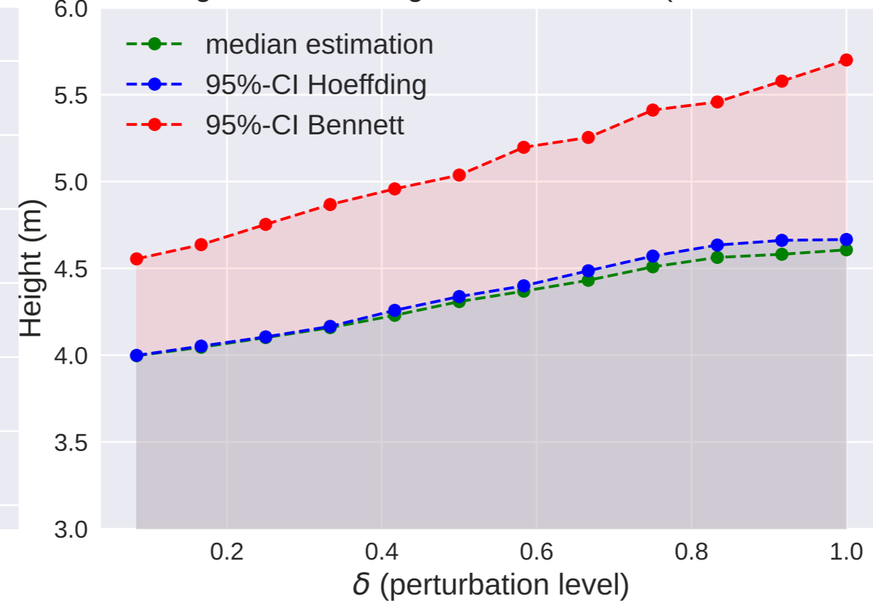
Hoeffding and Bennett right-sided 95%-CIs ( n=5000 , \alpha=0.95 )
