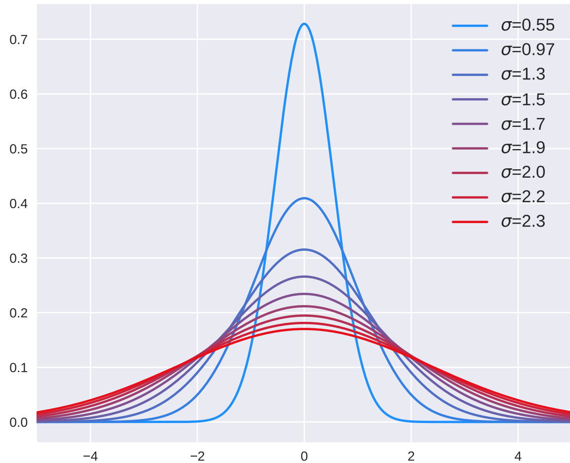
Non-truncated normal distributions
