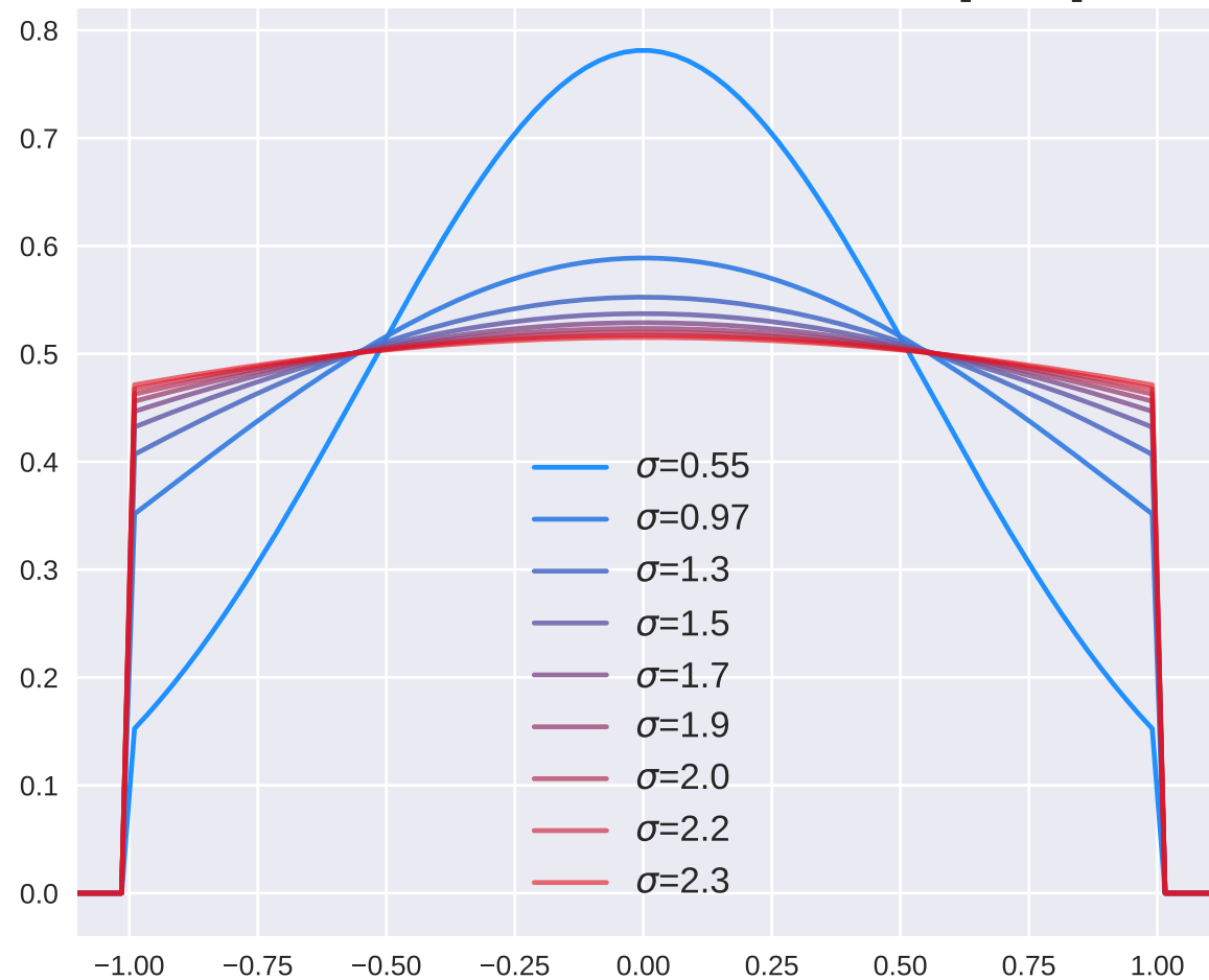
Truncated normal distributions on [-1, 1]
