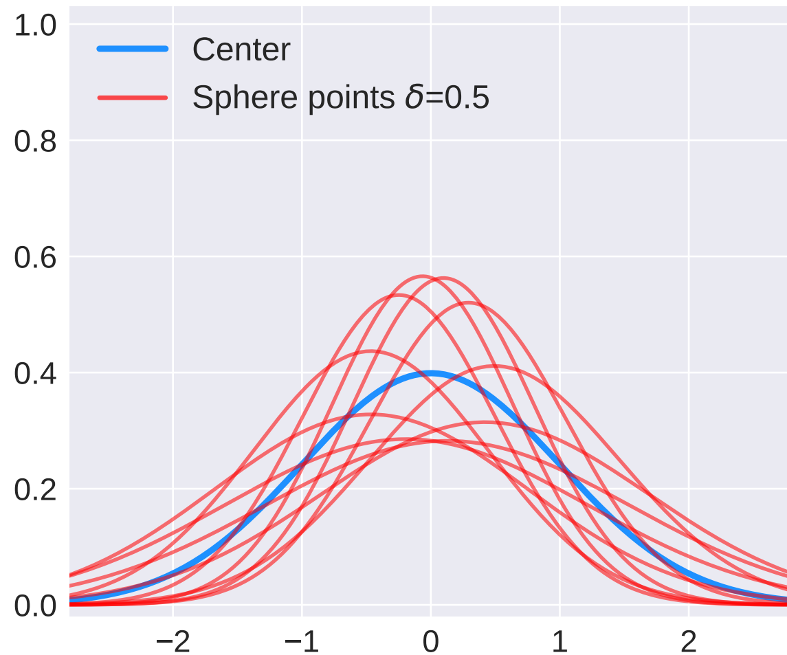
Normal distributions
