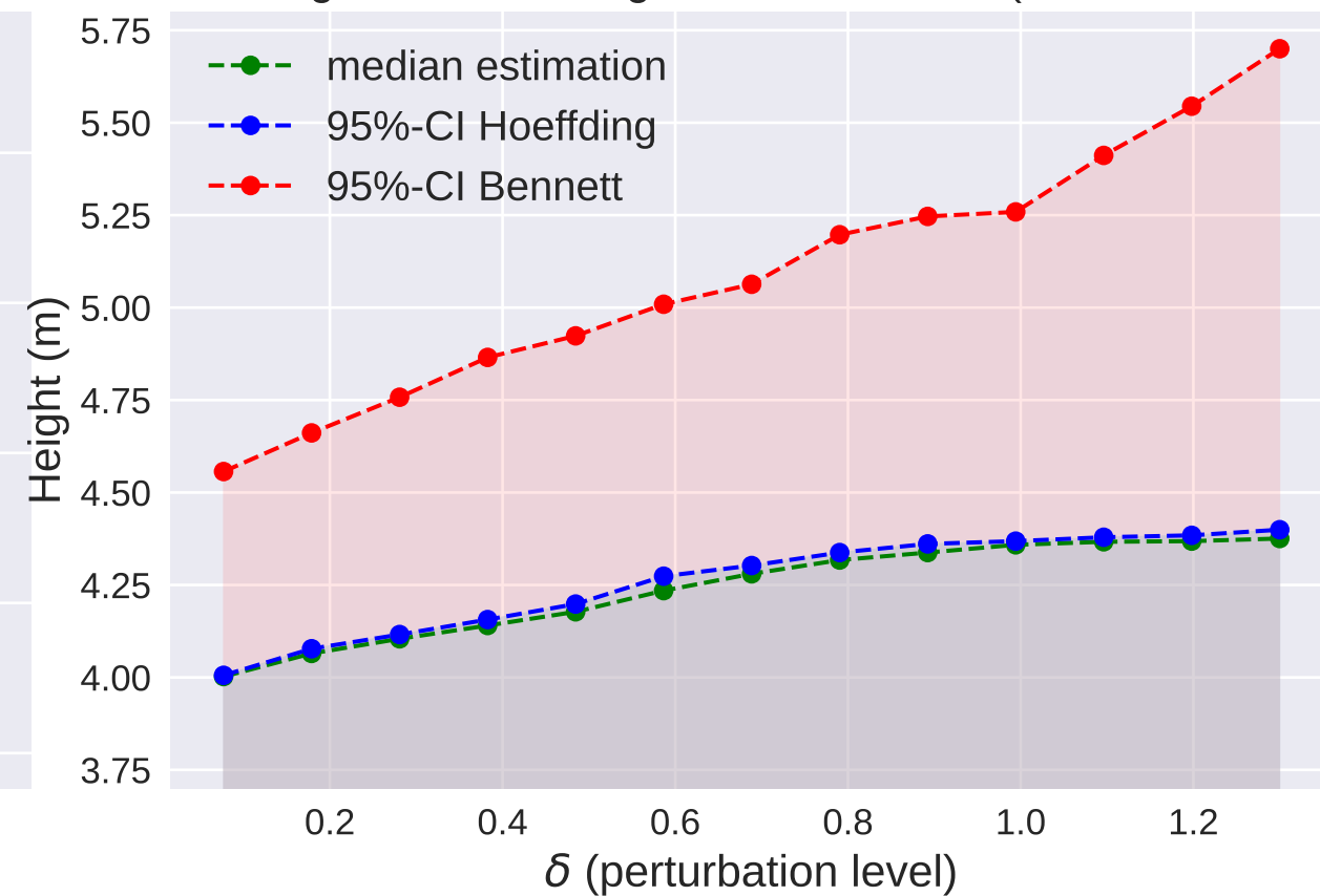
Hoeffding and Bennett right-sided 95%-CIs ( n=5000 , \alpha=0.95 )
