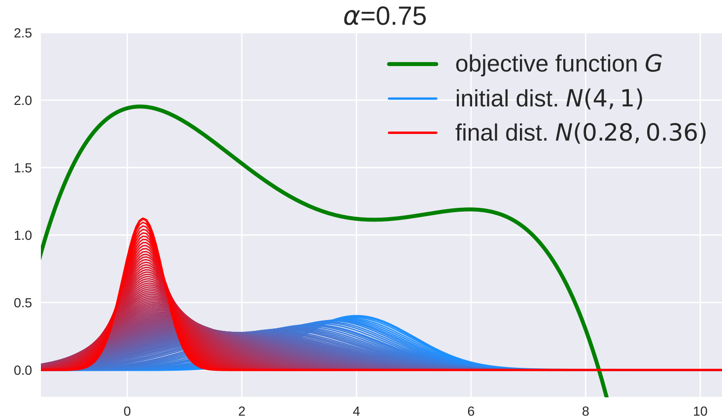
IGO-Q on a toy case (iterations=100, n=100 , \eta=0.2 ) with different \alpha
