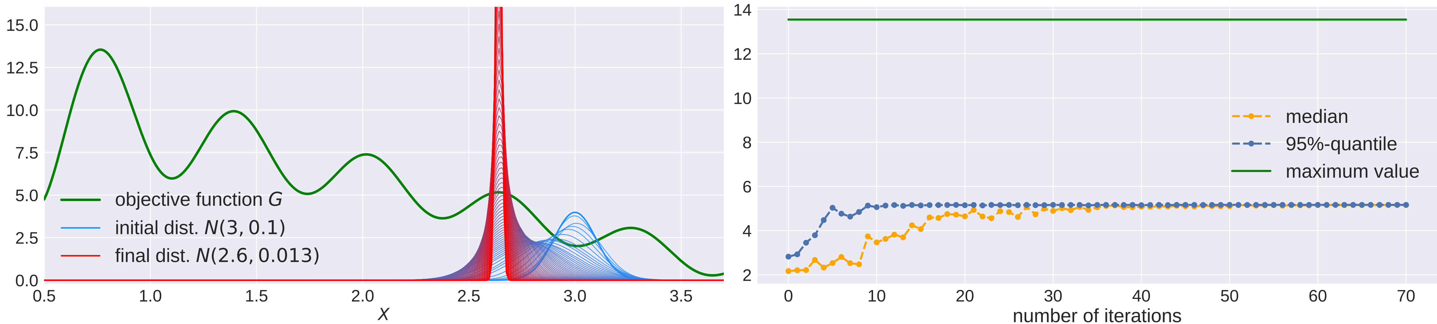
IGO-Q on a toy case (iterations=70, n=30 , \alpha=0.95 , \eta=1 )
