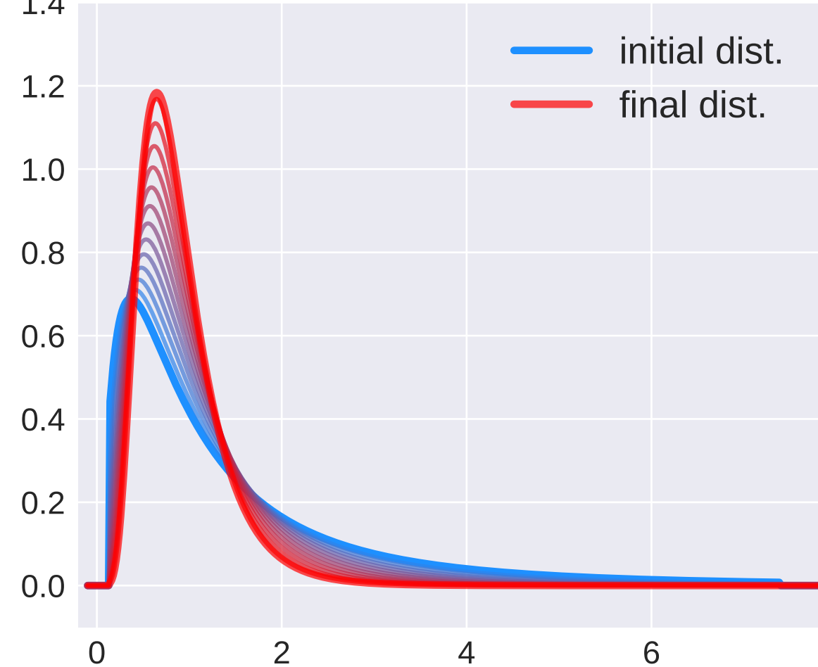
LogNormal distributions tr. on [e^{-2}, e^2]
