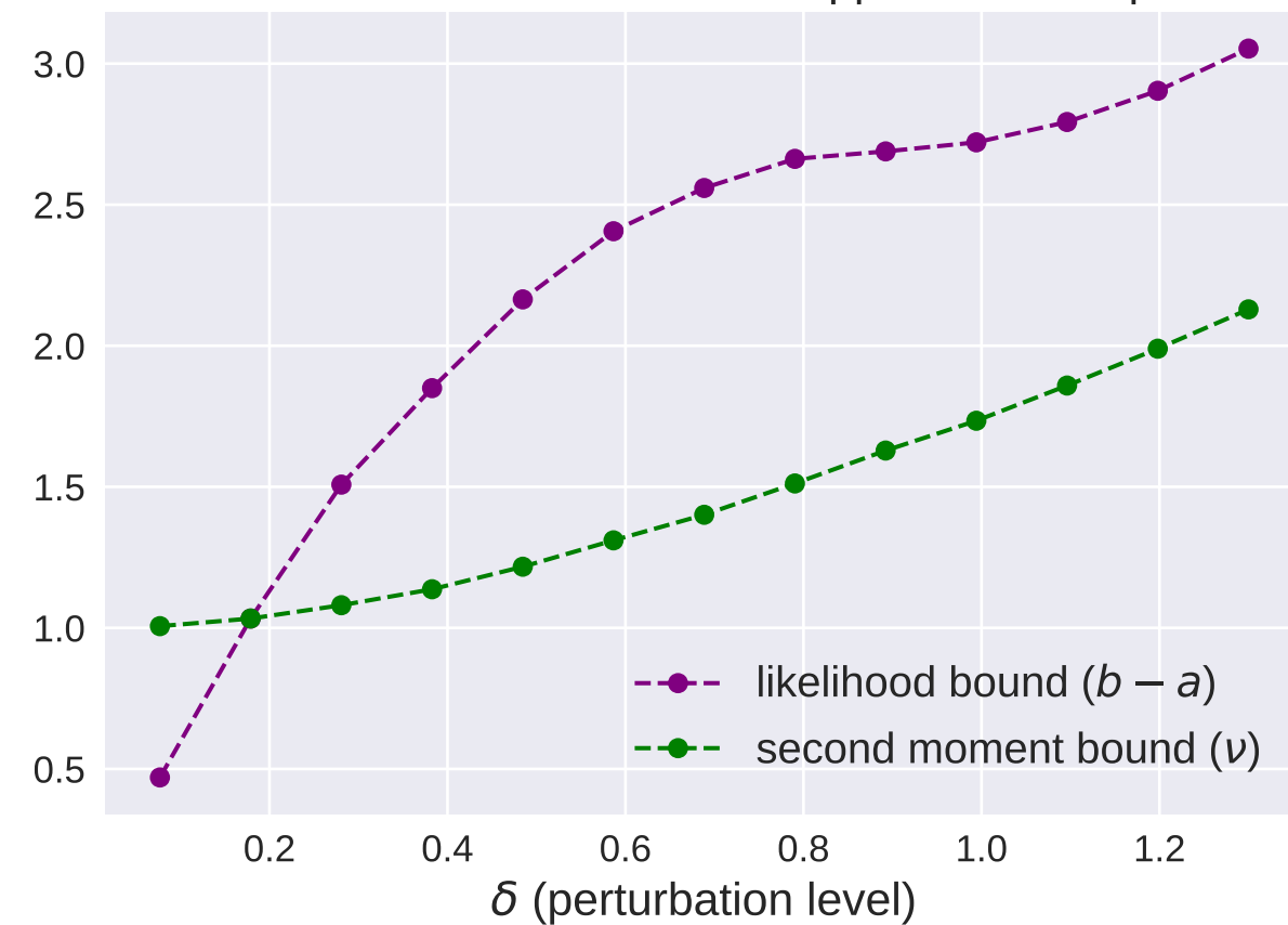
Likelihood second moment and support size comparison
