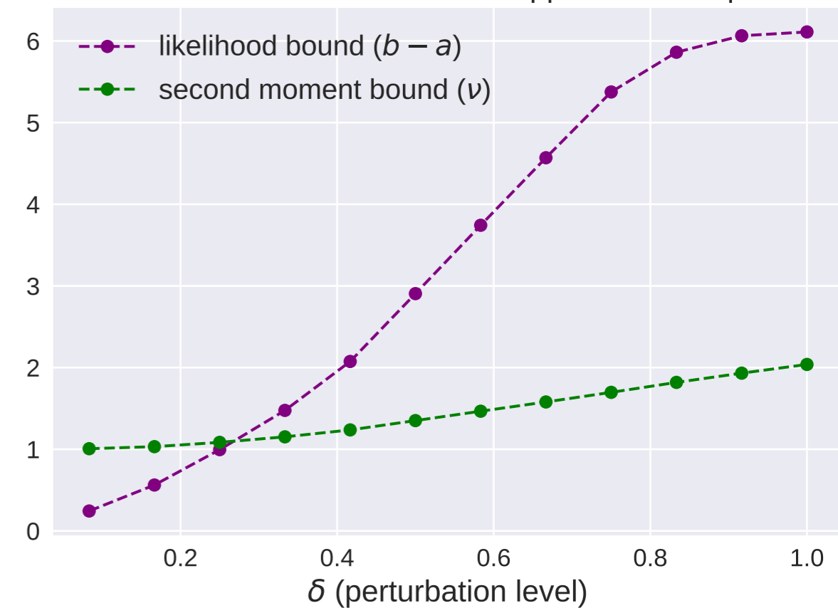
Likelihood second moment and support size comparison
