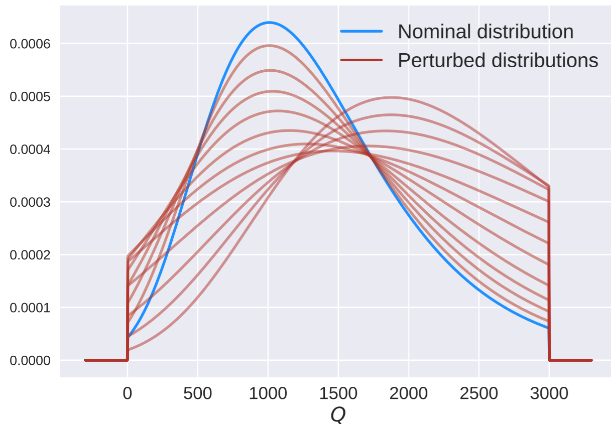
Perturbations of the nominal distribution
