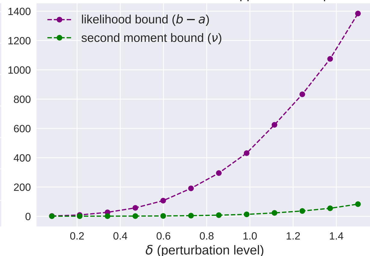
Likelihood second moment and support size comparison
