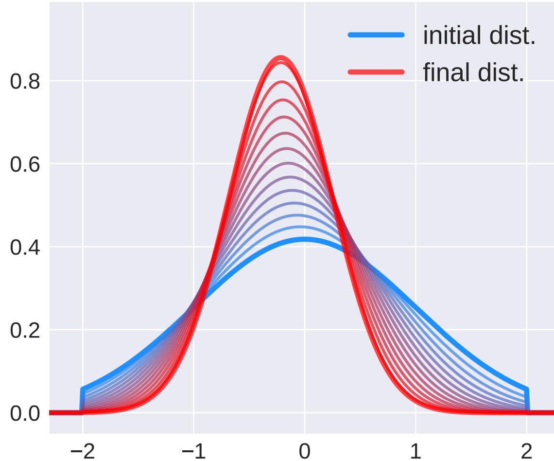
Normal distributions tr. on [-2, 2]
