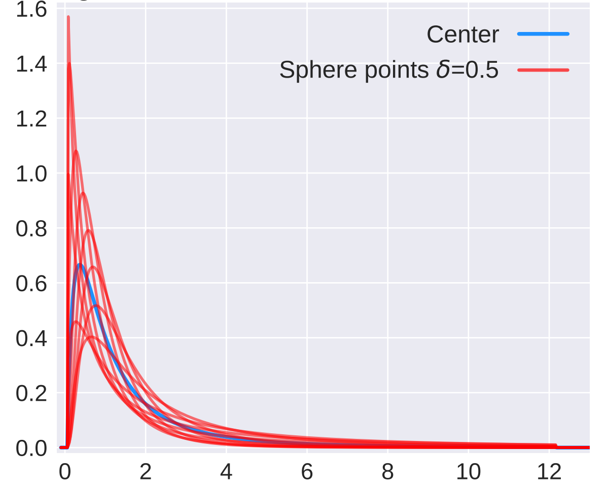
LogNormal distributions tr. on [e^{-2.5}, e^{2.5}]
