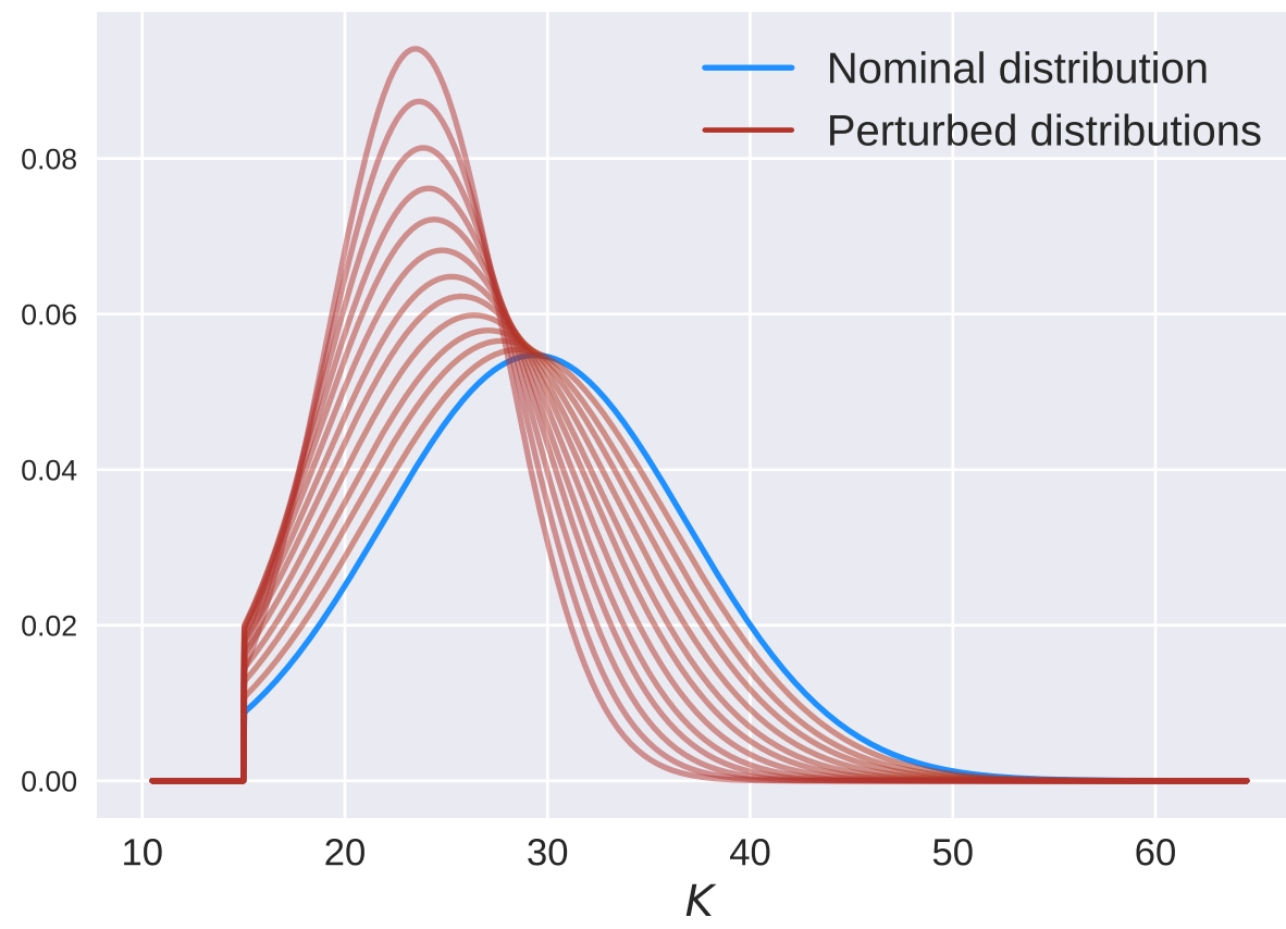
Perturbations of the nominal distribution
