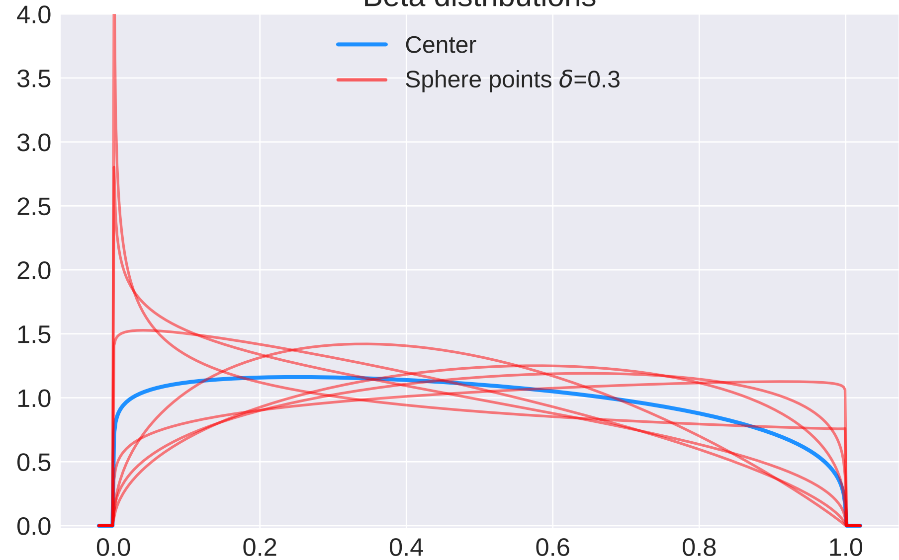
Beta distributions
