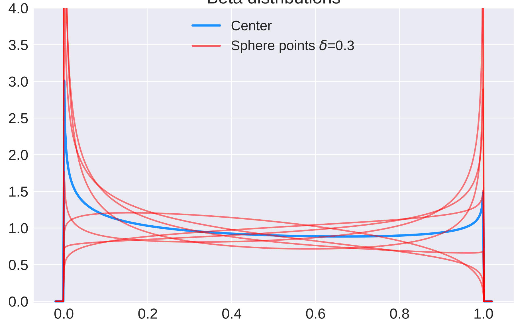
Beta distributions
