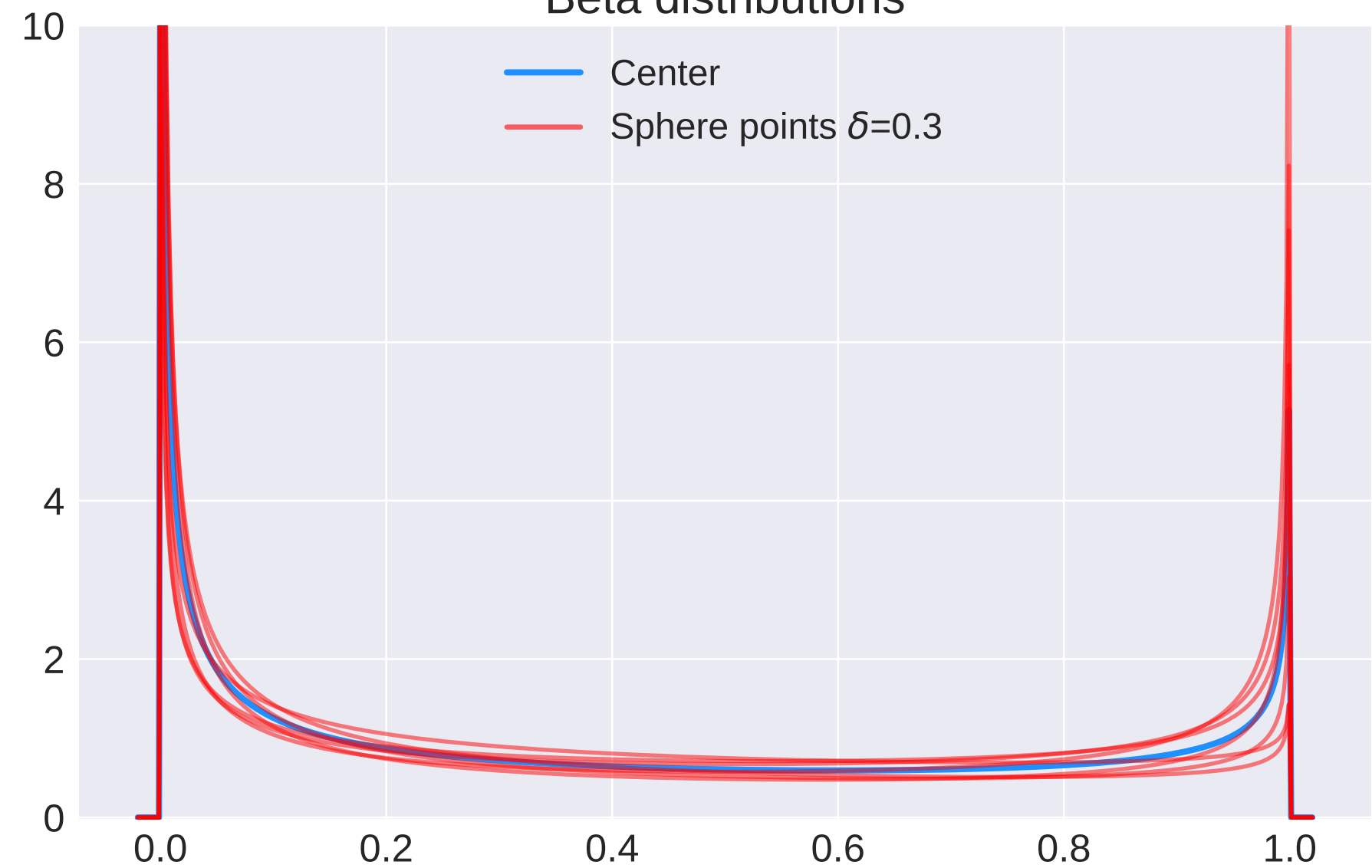
Beta distributions
