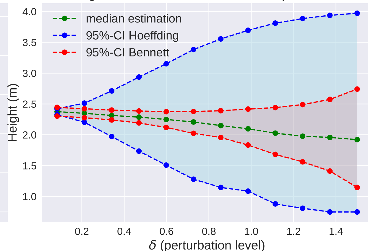
Hoeffding and Bennett two-sided 95%-CIs ( n=5000 , \alpha=0.5 )
