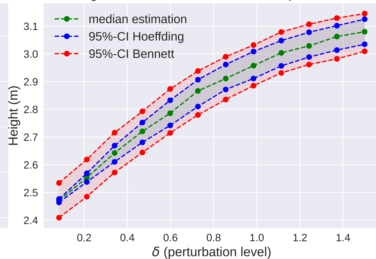
Hoeffding and Bennett two-sided 95%-CIs ( n=5000 , \alpha=0.5 )
