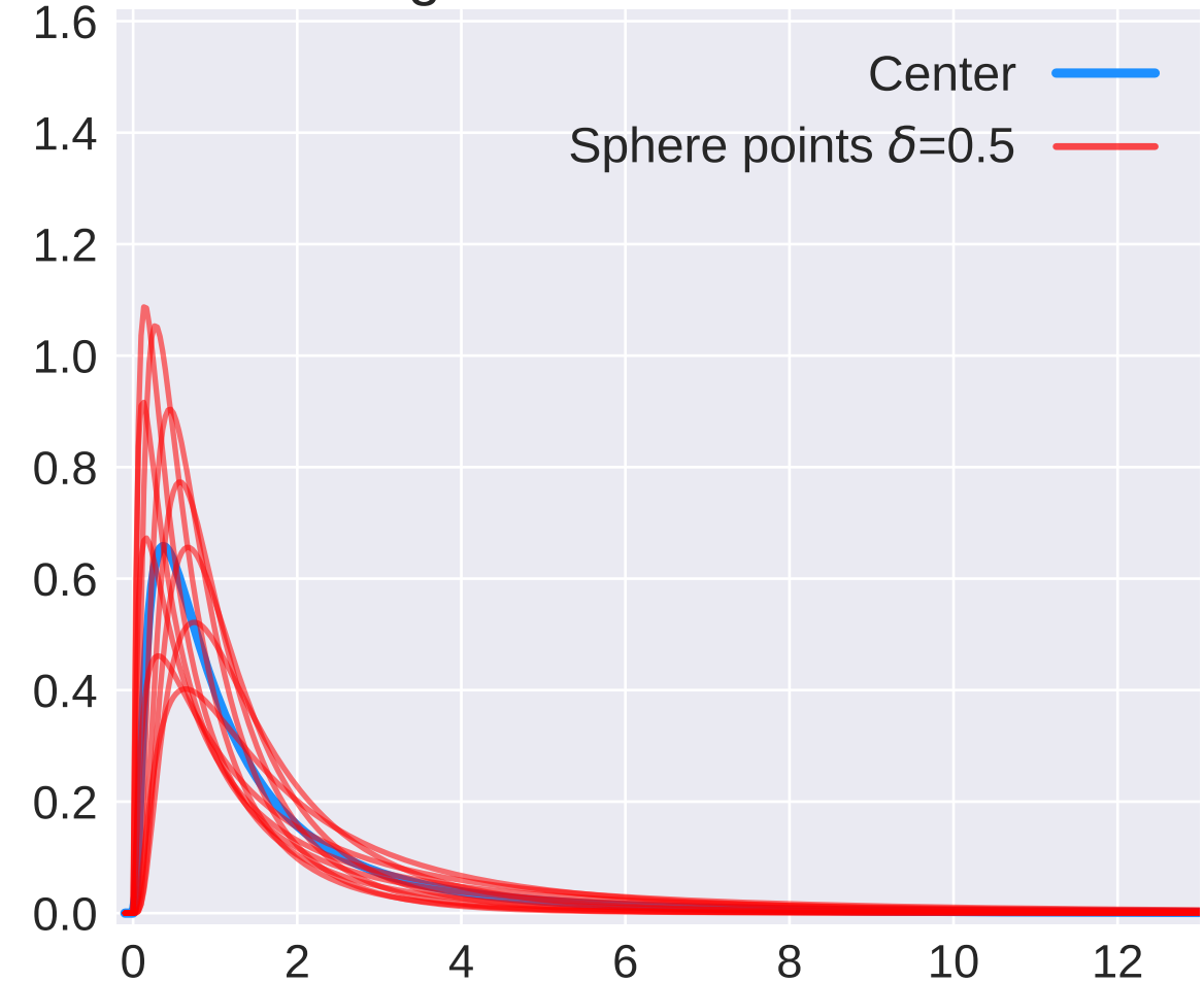
LogNormal distributions
