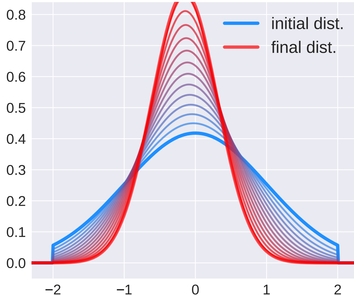
Normal distributions tr. on [-2, 2]
