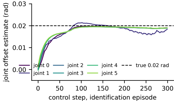
ALOHA transfer-cube, \pi_0 : +0.02 rad on six joints
