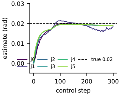
ALOHA, \pi_0 , +0.02 rad, left arm
