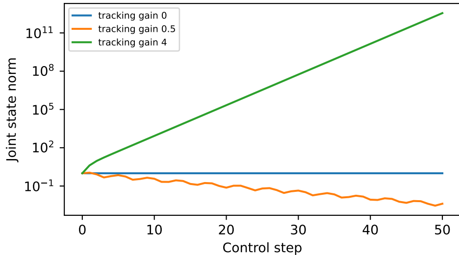
Joint feedback can stabilize a neutral mode
