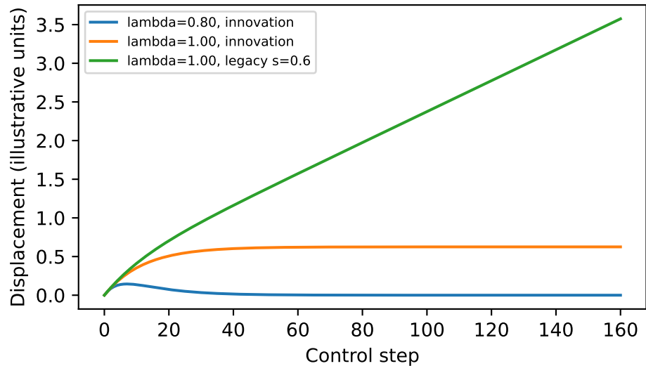
The same observer meets different execution memory
