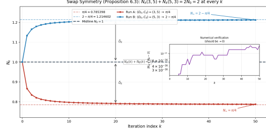
Figure 4: Swap symmetry (Proposition 6.3): the two runs (D_k, C_k) = (3, 5) and (5, 3) mirror around the midline N_k = 1 at every iteration k . Run A decreases monotonically to \pi/4 . Run B increases monotonically to 2 - \pi/4 . Equal brackets \delta_k confirm N_A(k) + N_B(k) = 2N_0 = 2 at each step. Inset: numerical residual |N_k + N_k - 2| is at floating-point zero throughout.
