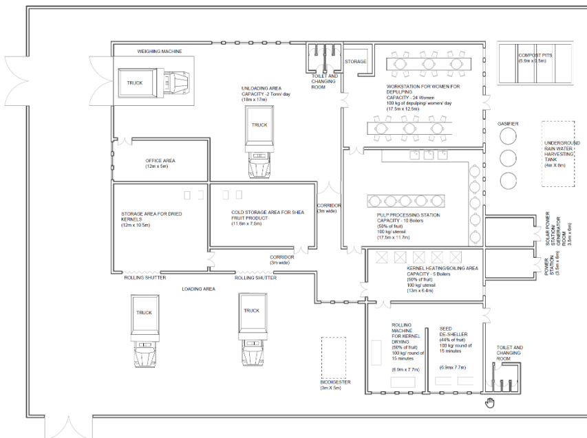
SHEA BUTTER COLLECTION UNIT LAYOUT - OPTION 02 CAPACITY - 2 TONNI/ DAY
