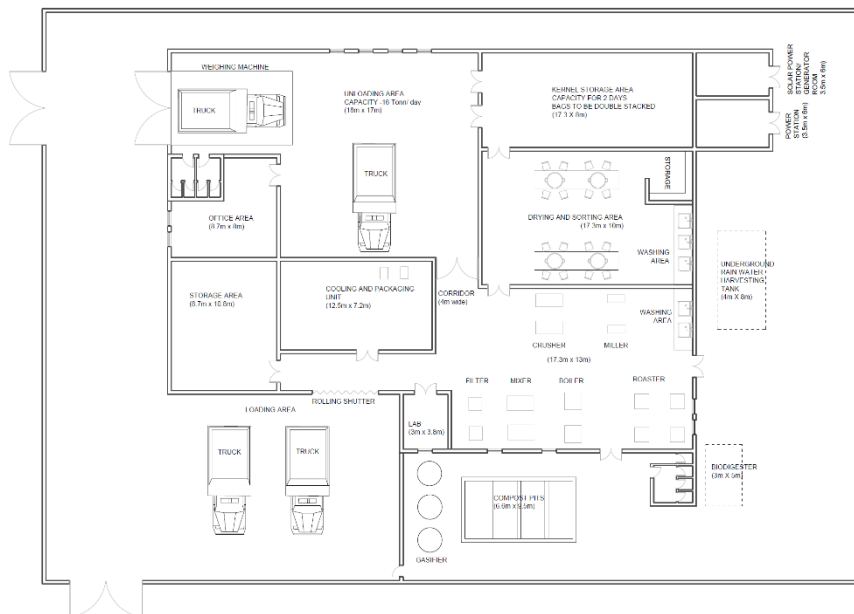
SHEA BUTTER PROCESSING UNIT LAYOUT CAPACITY - 16 TONNI/ DAY
