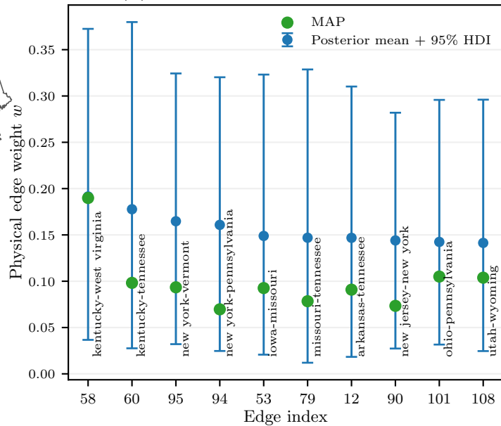
(c) Top 10 conductive edges
