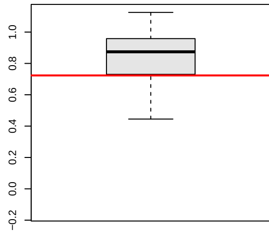
Predictions at one point, k = 5
