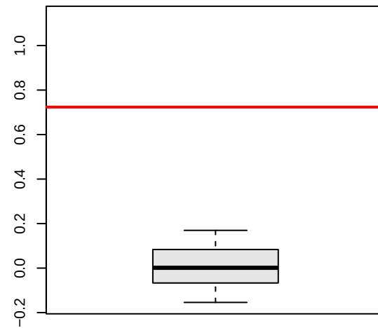
Predictions at one point, k = 150
