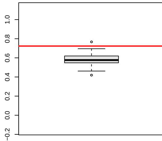
Predictions at one point, k = 40
