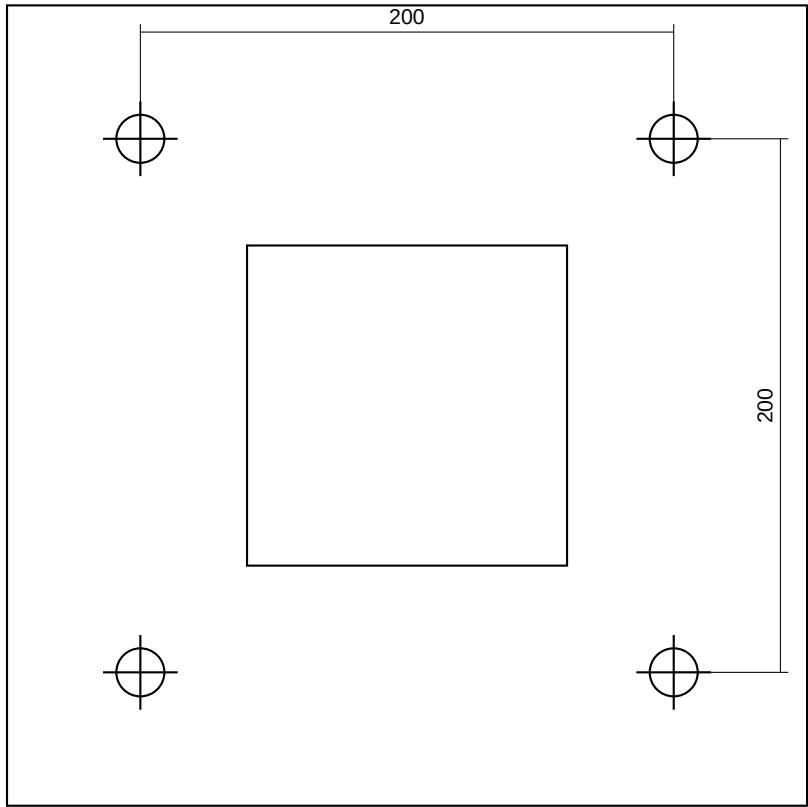
PLAN - 400x400x25 BASE PLATE WITH 4 No. M20 RODS
