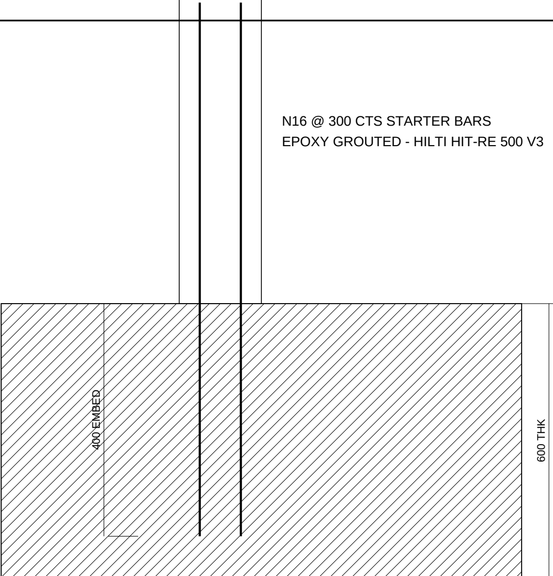
SECTION B-B - WALL TO EXISTING SLAB
