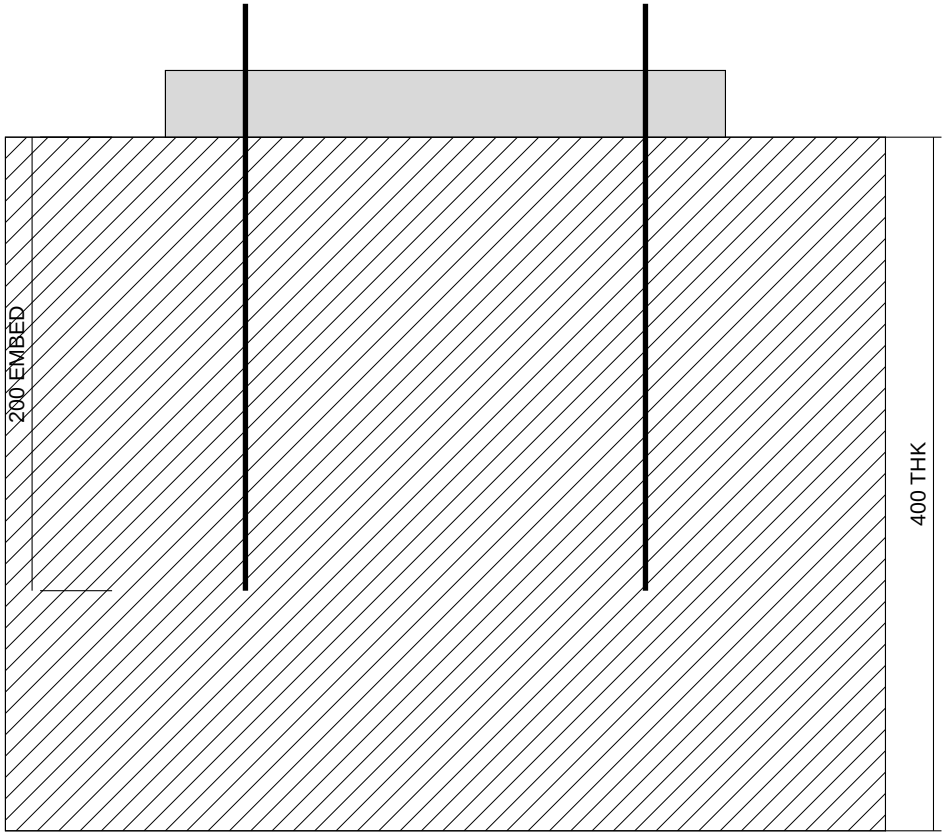
SECTION A-A - ANCHOR RODS IN 400 THK CONCRETE SLAB
