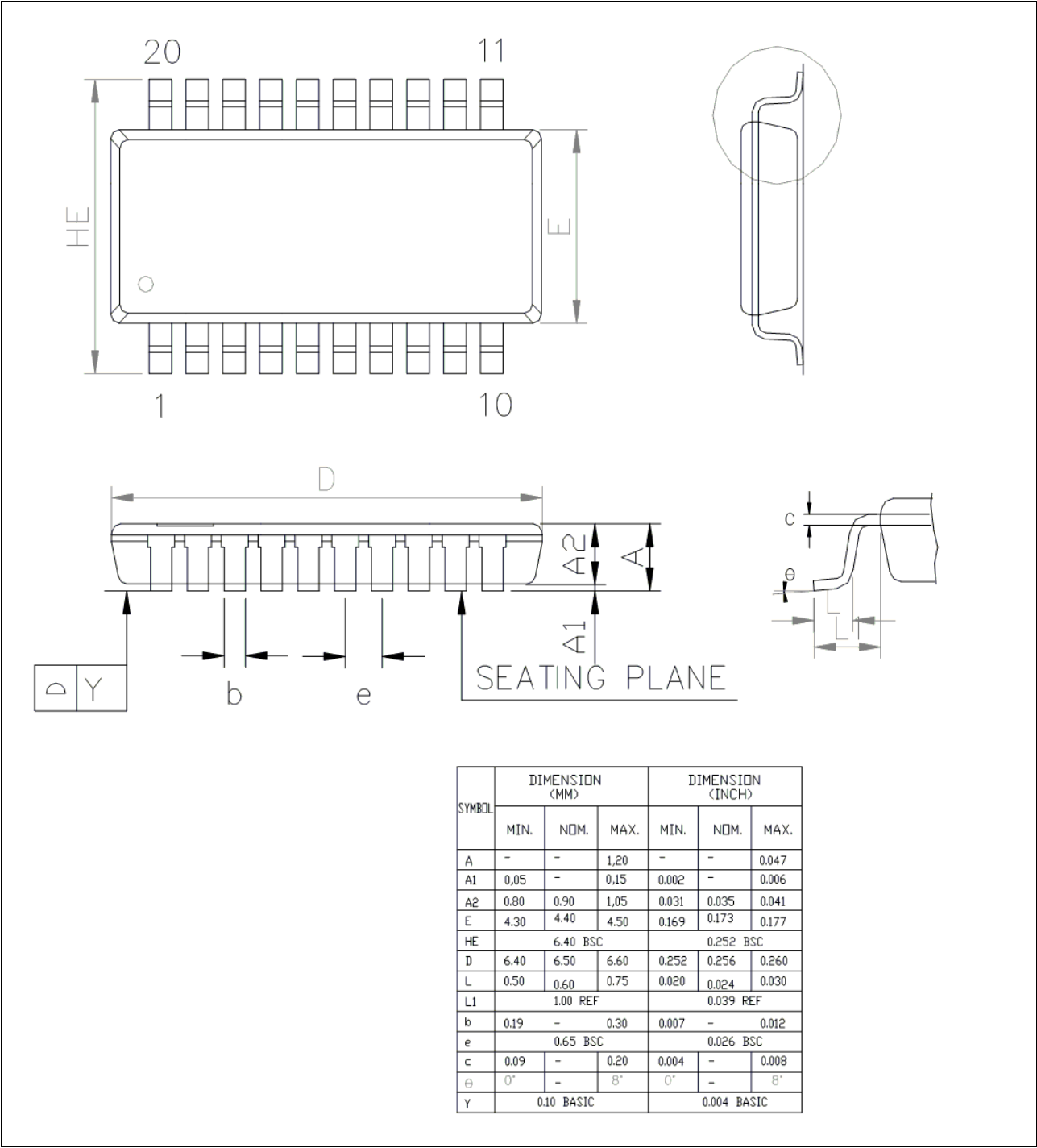
Figure 9.4-1 TSSOP-20 Package Dimension
