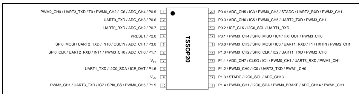
Figure 4.1-4 Pin Assignment of TSSOP20 Package
