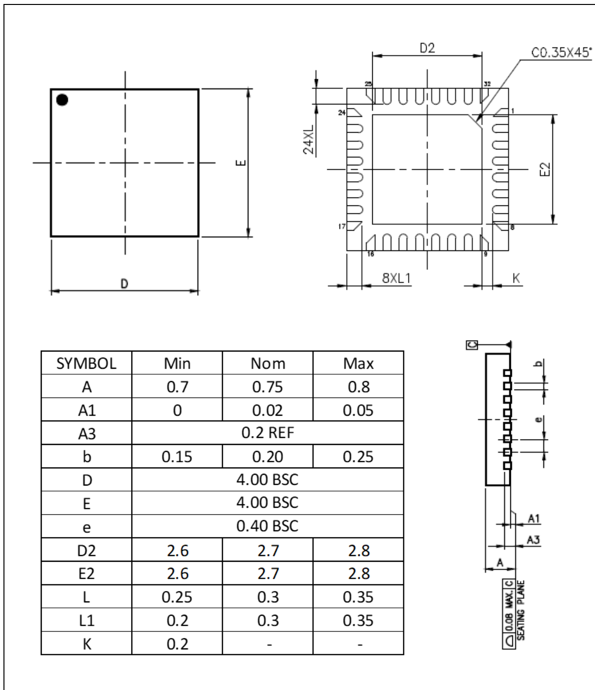
Figure 9.1-1 QFN-32 Package Dimension
